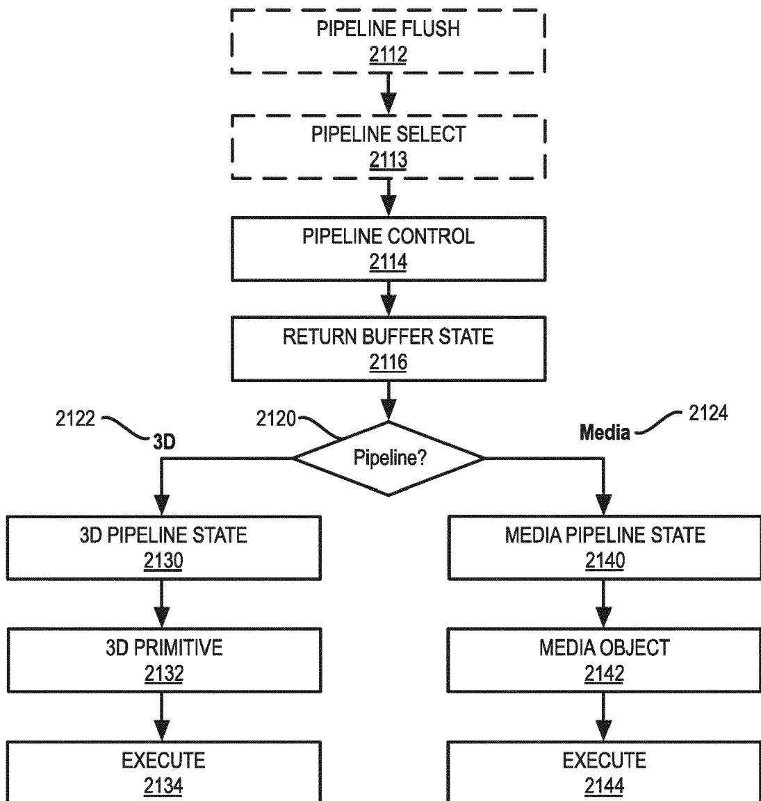
FIG. 21B GRAPHICS PROCESSOR COMMAND SEQUENCE 2110
