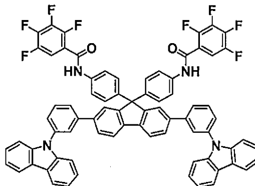
Fluorine Atom-Containing Compound C
