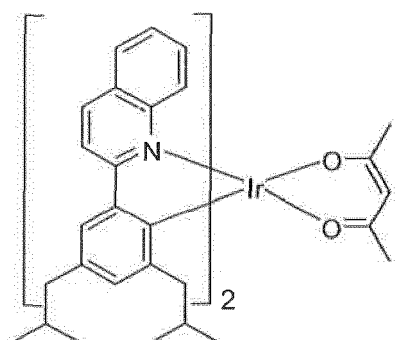
Compound 4
