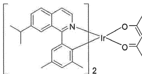
Compound 9
