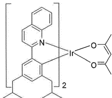
Compound 4
