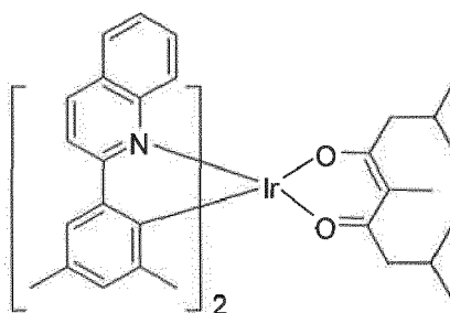
Compound 5
