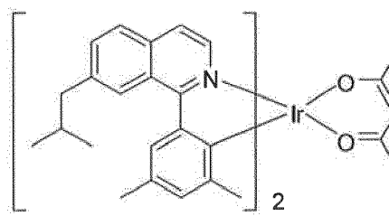
Compound 10
