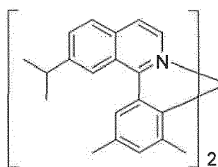
Compound 9
