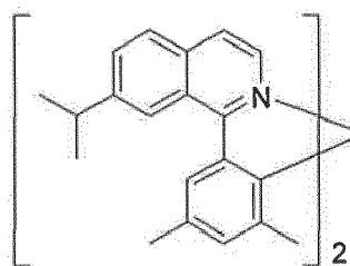
Compound 9
