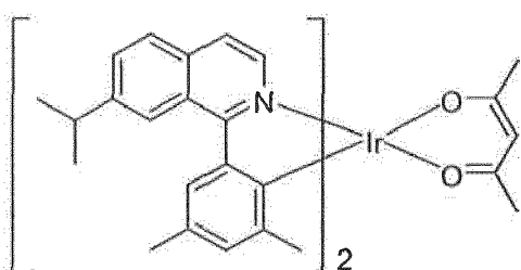
Compound 9
