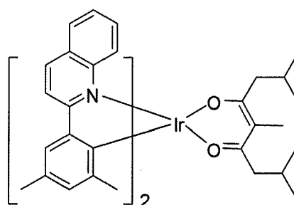
Compound 5
