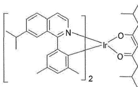
Compound 7
