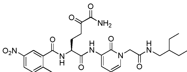
(S)- N 1 -(1-(2-(2-ethylbutylamino)-2-oxoethyl)-2-oxo-1,2-dihydropyridin-3-yl)-2-(2-methyl-5-nitrobenzamido)-5-oxohexanediamide
