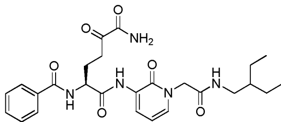
(S)-2-benzamido- N 1 -(1-(2-(2-ethylbutylamino)-2-oxoethyl)-2-oxo-1,2-dihydropyridin-3-yl)-5-oxohexanediamide
