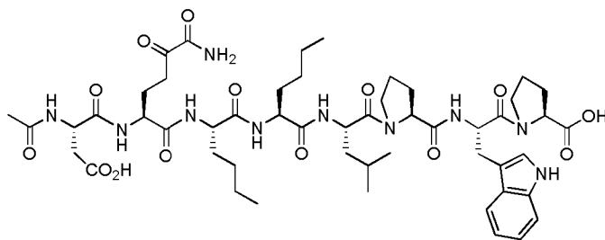
(S)-1-((S)-2-((S)-1-((4S,7S,10S,13S,16S)-7-(4-amino-3,4-dioxobutyl)-10,13-dibutyl-4-(carboxymethyl)-18-methyl-2,5,8,11,14-pentaoxo-3,6,9,12,15-pentaazonadecanecarbonyl)pyrrolidine-2-carboxamido)-3-(1H-indol-3-yl)propanoyl)pyrrolidine-2-carboxylic acid Chemical Formula: C_{51}H_{74}N_{10}O_{14} Exact Mass: 1050,54 Molecular Weight: 1051,19
