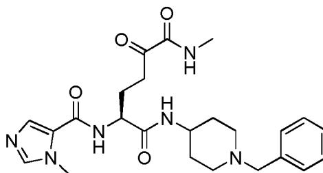
(S)-N 1 -(1-benzylpiperidin-4-yl)-N 6 -methyl-2-(1-methyl-1H-imidazole-5-carboxamido)-5-oxohexanediamide
