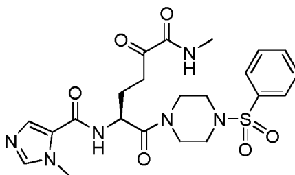
(S)-1-methyl-N-(6-(methylamino)-1,5,6-trioxo-1-(4-(phenylsulfonyl)piperazin-1-yl)hexan-2-yl)-1H-imidazole-5-carboxamide
