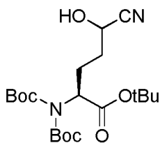
(2S)-tert-butyl 2-(bis(tert-butoxycarbonyl)amino)-5-cyano-5-hydroxypentanoate
