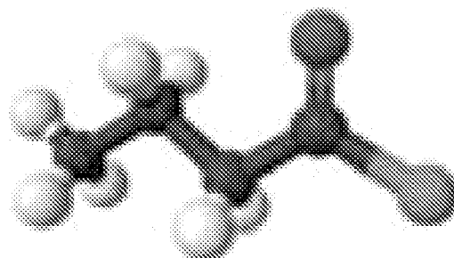
butyryl chloride
