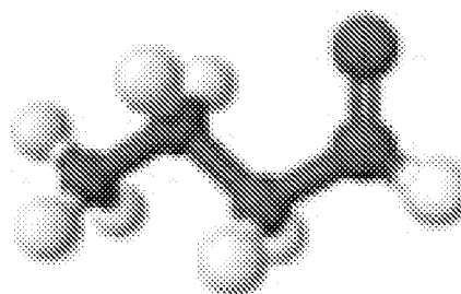
butyraldehyde
