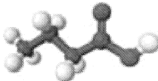
butyric acid
