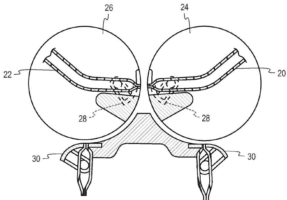
Fig. 2 Prior Art
