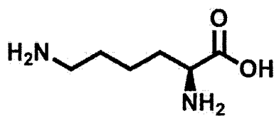
lysine
