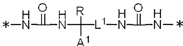
Formula (A)
