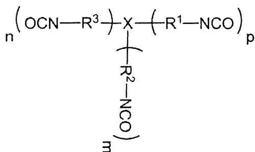
Formula (11)
