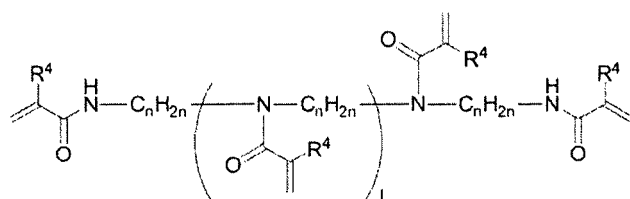
Formula (c)
