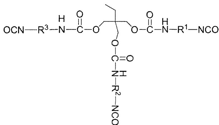
Formula (11A-1)
