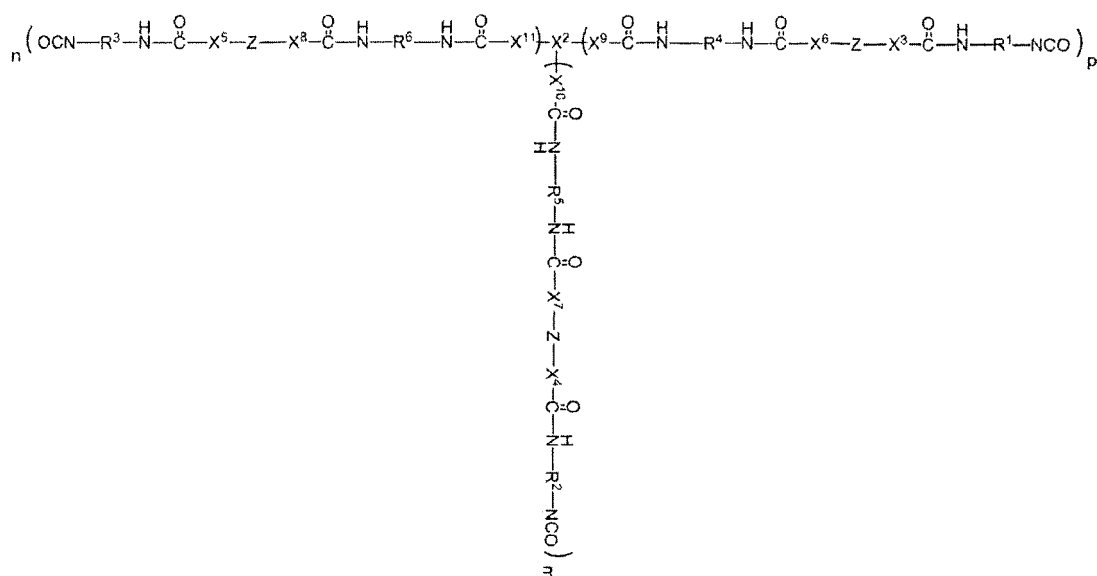
Formula (11B)
