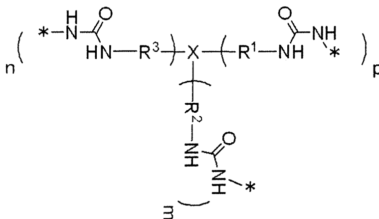
Structure (1)
