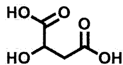
malic acid
