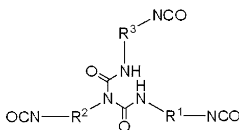
Formula (11D)
