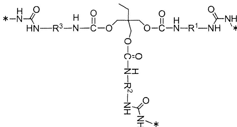
Structure (2)
