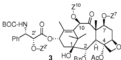
general structure of docetaxel derivatives
