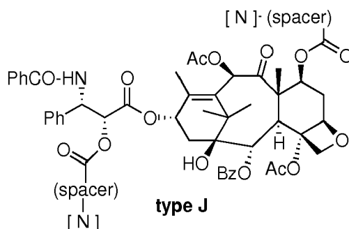
diester derivative of paclitaxel
