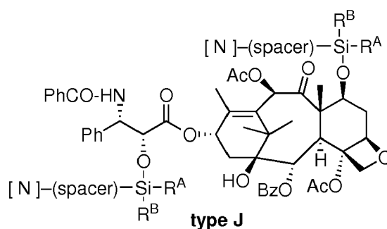
bis-silyl ether derivative of paclitaxel
