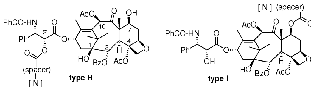
monoester derivatives of paclitaxel
