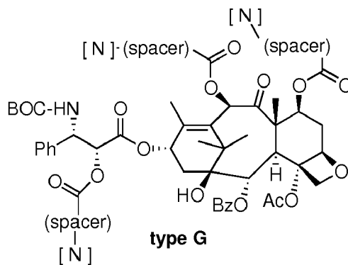
triester derivative of docetaxel
