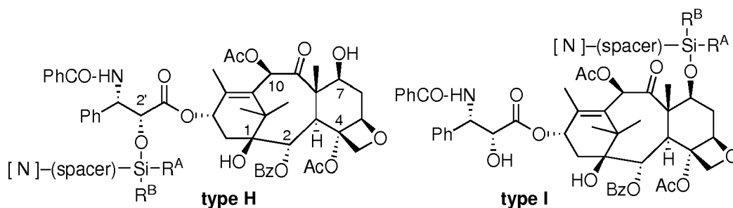
mono- silyl ether derivatives of paclitaxel
