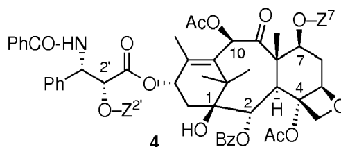
general structure of paclitaxel derivatives
