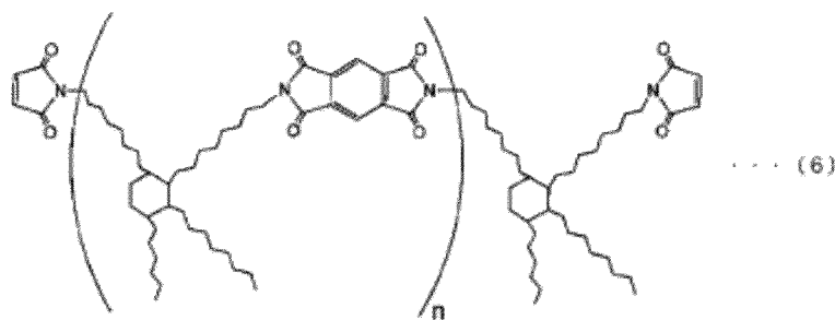
[Chemical formula 4]
