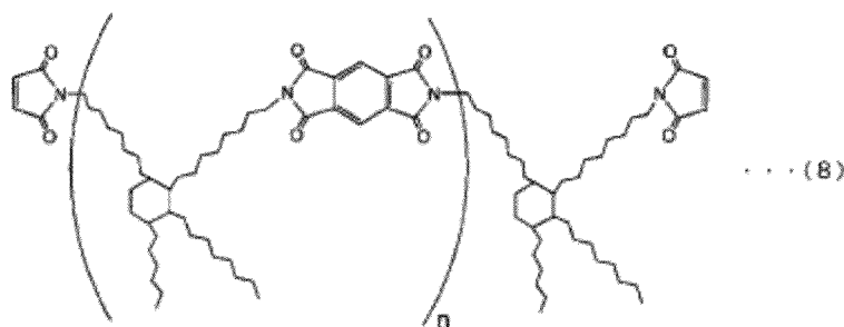
[Chemical formula 6]
