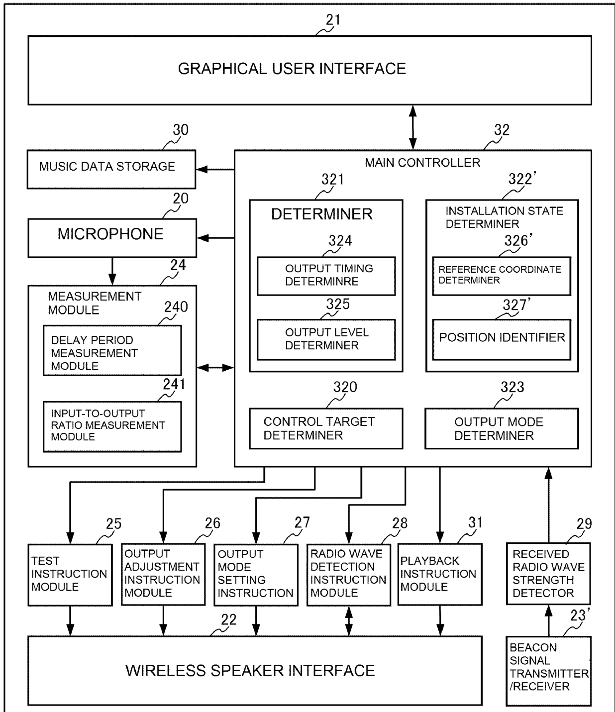
CONTROLLER 2'
