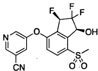
Compound 342
