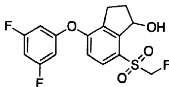
(R)-4-(3,5-Difluorophenoxy)-7-((fluoromethyl)sulfonyl)-2,3-dihydro-1H-inden-1-ol (Compound 59)
