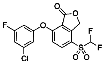
7-(3-Chloro-5-fluorophenoxy)-4-((difluoromethyl)sulfonyl)isobenzofuran-1(3H)-one ( Compound 84 )
