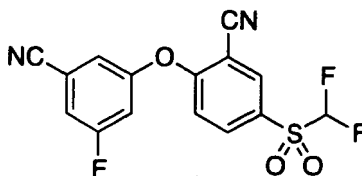
2-(3-Cyano-5-fluorophenoxy)-5-((difluoromethyl)sulfonyl)benzonitrile ( Compound 134 )
