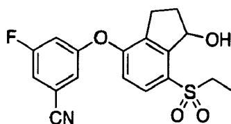
3-((7-(Ethylsulfonyl)-1-hydroxy-2,3-dihydro-1H-inden-4-yl)oxy)-5-fluorobenzonitrile ( Compound 205 )
