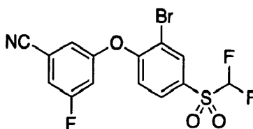
3-(2-Bromo-4-((difluoromethyl)sulfonyl)phenoxy)-5-fluorobenzonitrile ( Compound 132 )
