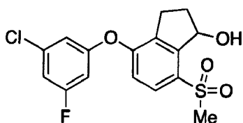
4-(3-Chloro-5-fluorophenoxy)-7-(methylsulfonyl)-2,3-dihydro-1H-inden-1-ol ( Compound 90 )
