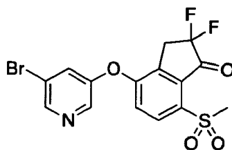
4-((5-Bromopyridin-3-yl)oxy)-2,2-difluoro-7-(methylsulfonyl)-2,3-dihydro-1H-inden-1-one ( Compound 323 )
