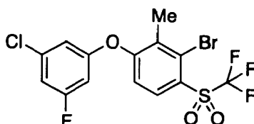
3-Bromo-1-(3-chloro-5-fluoro-phenoxy)-2-methyl-4-(trifluoromethylsulfonyl)benzene ( Compound 140 )
