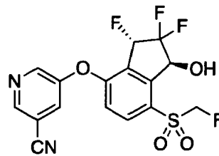
Compound 345
