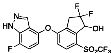
2,2-Difluoro-4-((7-fluoro-1H-indazol-4-yl)oxy)-7-((trifluoromethyl)sulfonyl)-2,3-dihydro-1H-inden-1-ol ( Compound 241 )
