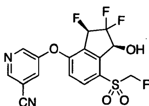
Compound 344
