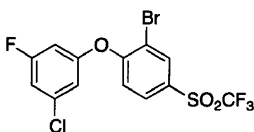
2-Bromo-1-(3-chloro-5-fluorophenoxy)-4-((trifluoromethyl)sulfonyl)benzene ( Compound 116 )
