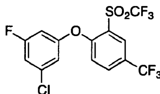
1-(3-Chloro-5-fluorophenoxy)-4-(trifluoromethyl)-2-((trifluoromethyl)sulfonyl)benzene ( Compound 129 )
