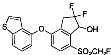
4-(Benzo[b]thiophen-4-yloxy)-2,2-difluoro-7-((fluoromethyl)sulfonyl)-2,3-dihydro-1H-inden-1-ol ( Compound 242 )
