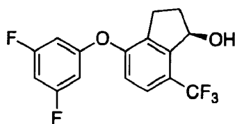
(R)-4-(3,5-Difluorophenoxy)-7-(trifluoromethyl)-2,3-dihydro-1H-inden-1-ol (Compound 58)
