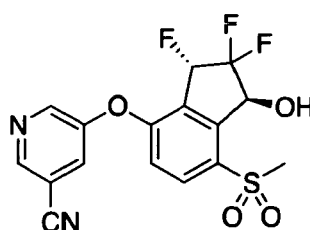
Compound 343
