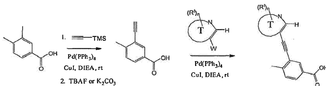
Scheme XIX
