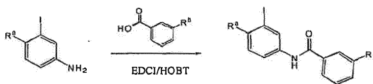
Scheme IX
