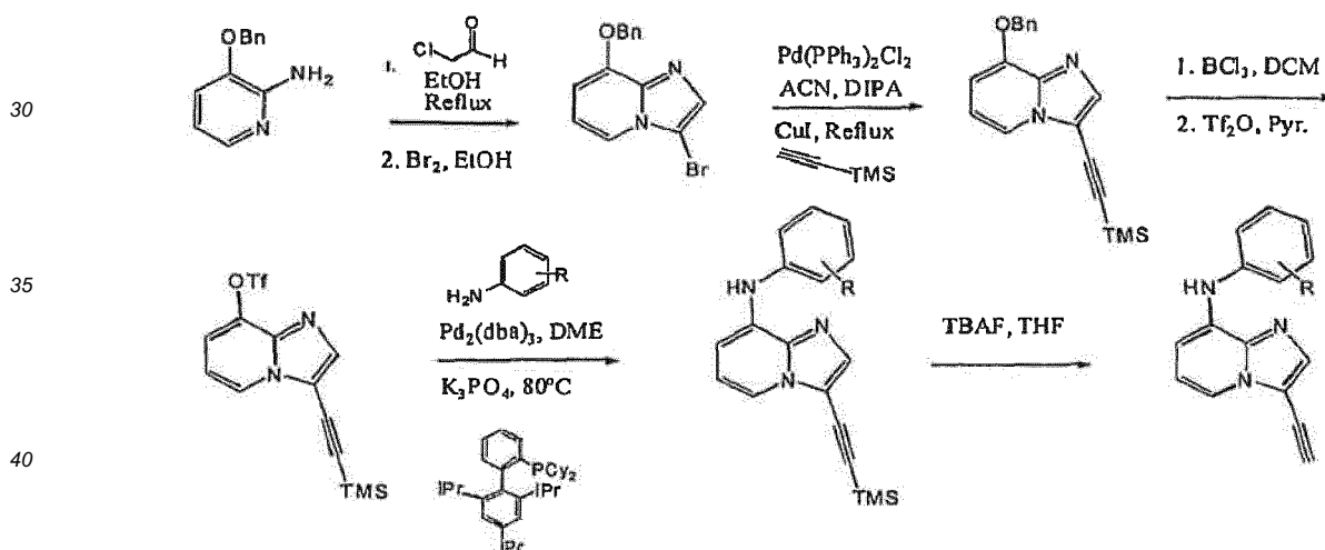
Scheme VI: Preparation of C-8 Amino Substituted 3-Ethynylimidazo[1,2-a]pyridines
