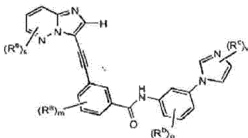
Formula IIc.
