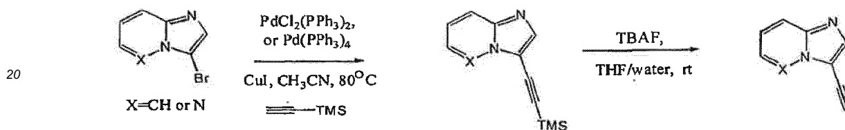
Scheme V: Preparation of 3-Ethynylimidazo[1,2-a]pyridine or 3-Ethynylimidazo[1,2-b]pyridazine
