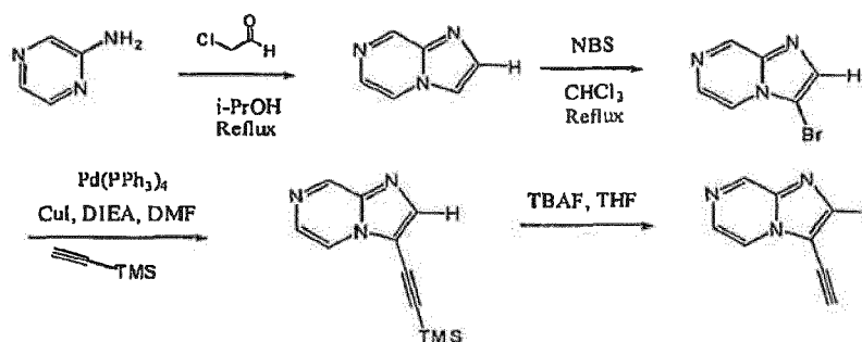
Scheme III: Preparation of 3-Ethynylimidazo[1,2-a]pyrazine
