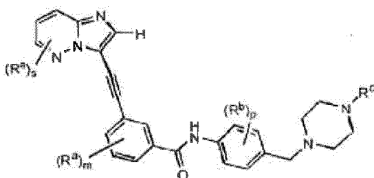
Formula IIIc
