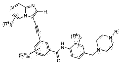
Formula IIIa
