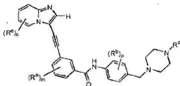
Formula IIIb
