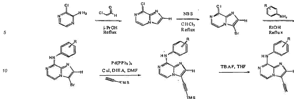
Scheme IV: Preparation of C-8 Substituted 3-Ethynylimidazo[1,2-a]pyrazines
