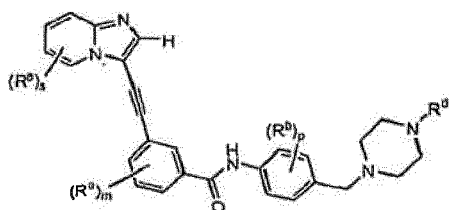
Formula IIlb
