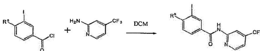
Scheme X
