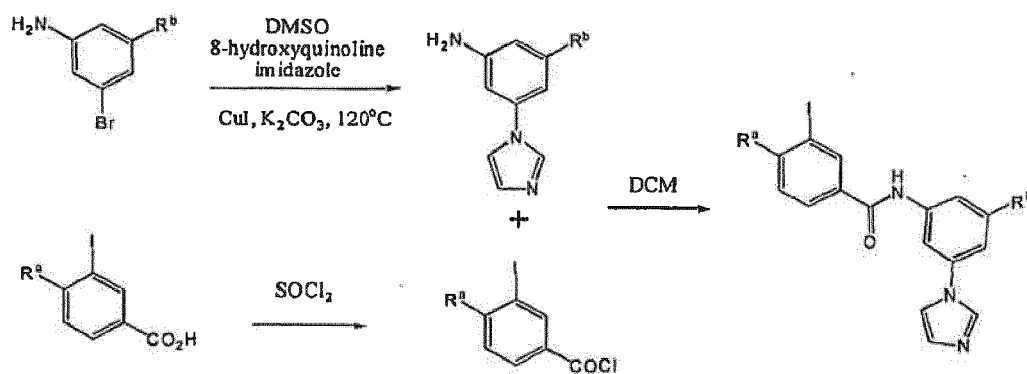
Scheme XI
