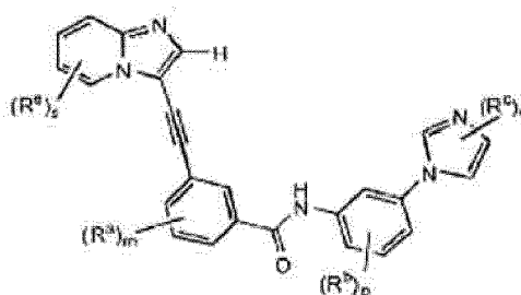
Formula IIb
