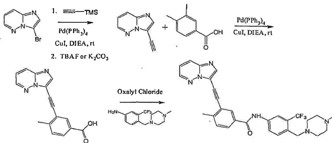
Scheme XVIII
