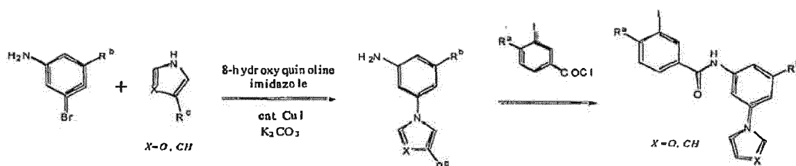
Scheme XII
