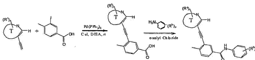
Scheme XVII
