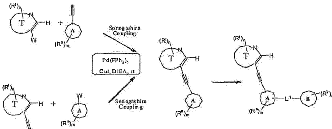
Scheme XVI
