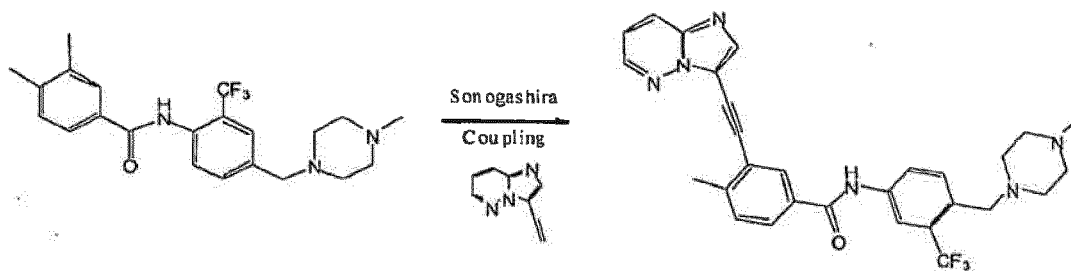
Scheme XIV
