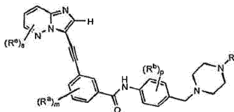
Formula IIIc
