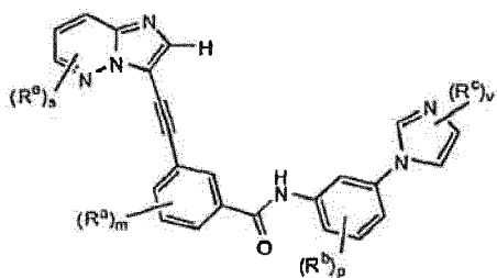
Formula IIc
