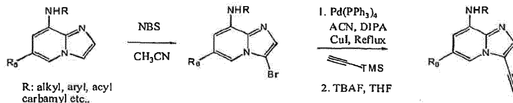
15 Scheme VIII: Preparation of C-6 and C-8 Substituted 3-Ethynylimidazo [1,2-a] pyridines.
