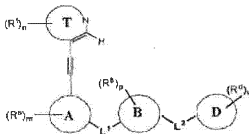
Formula III
