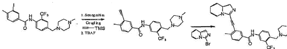
Scheme XV
