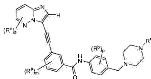
Formula IIIc
