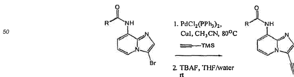
Scheme VII: Preparation of C-8 substituted 3-Ethynylimidazo[1,2-a]pyridines
