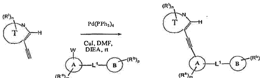
Scheme I: Sonogashira Coupling Reaction
