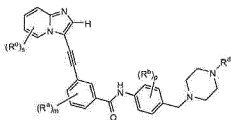
Formula IIIb
