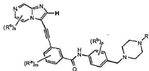
Formula IIIa
