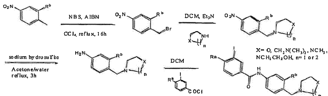
Scheme XIII
