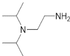
\text{N}_1, \text{N}_1 -diisopropylethane-1,2-diamine
