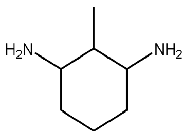
2-methylcyclohexane-1,3-diamine,
