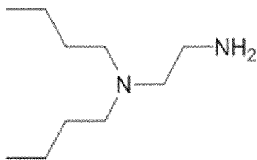
N,N'-dibutylethane-1,2-diamine
