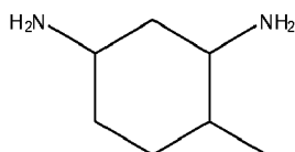
4-methylcyclohexane-1,3-diamine,
