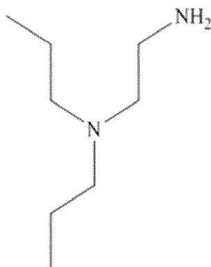
N,N'-dipropylpropane 1,3 diamine
