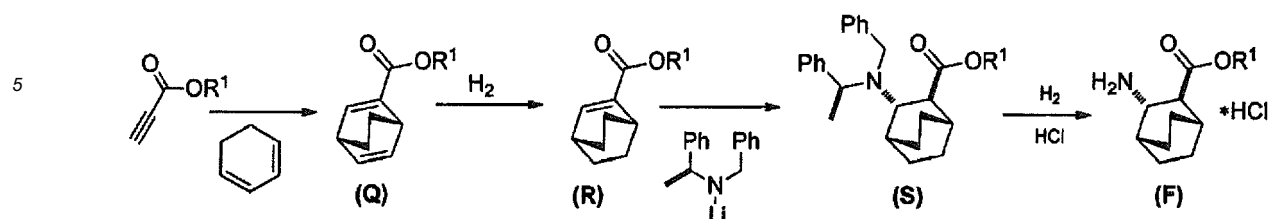
Scheme 6:
