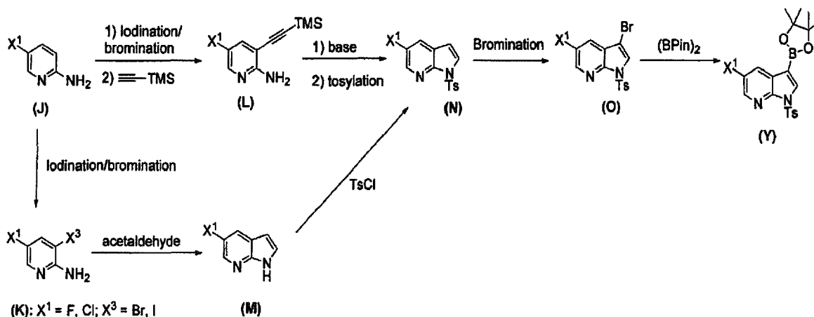
Scheme 10:
