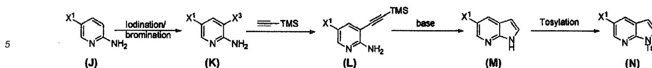
Scheme 8:
