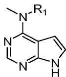
Formula I.
