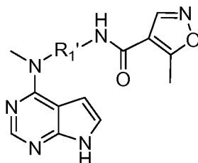
Formula I-b
