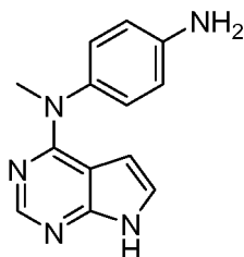
Compound 1
