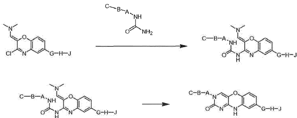
[0166] Scheme 2c - [6,6,6] isocytosines
