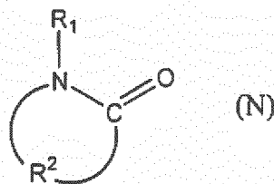
[Chemical Formula 2]
