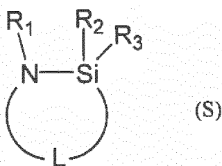
[Chemical Formula 1]
