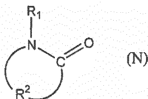
[Chemical Formula 1]
