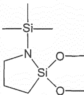
[Chemical Formula 4]
