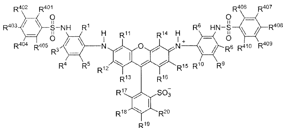
Formula (2)
