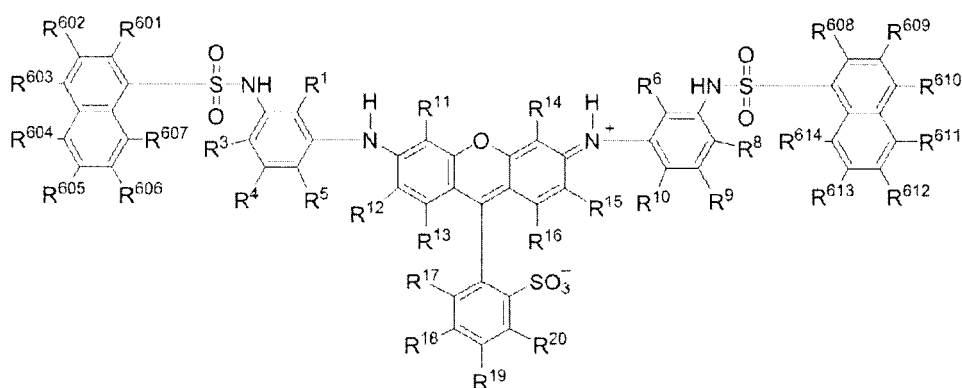
Formula (4)
