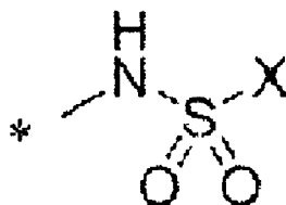
Formula (A)
