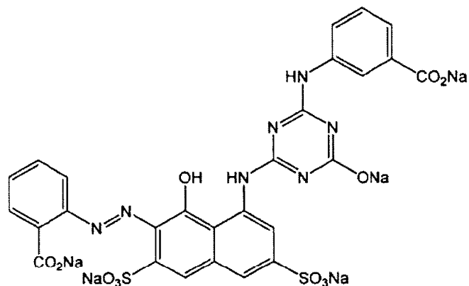
(Compound 2-Y)
