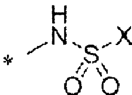
Formula (A)
