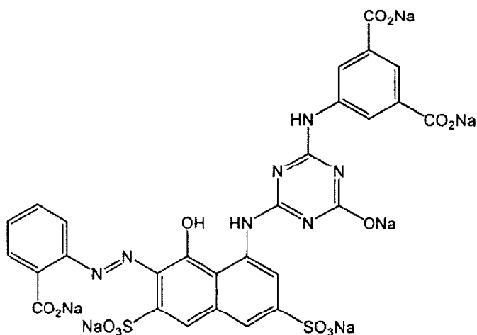
(Compound 2-Z)
