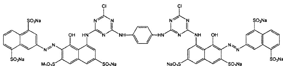
(Compound Z)
