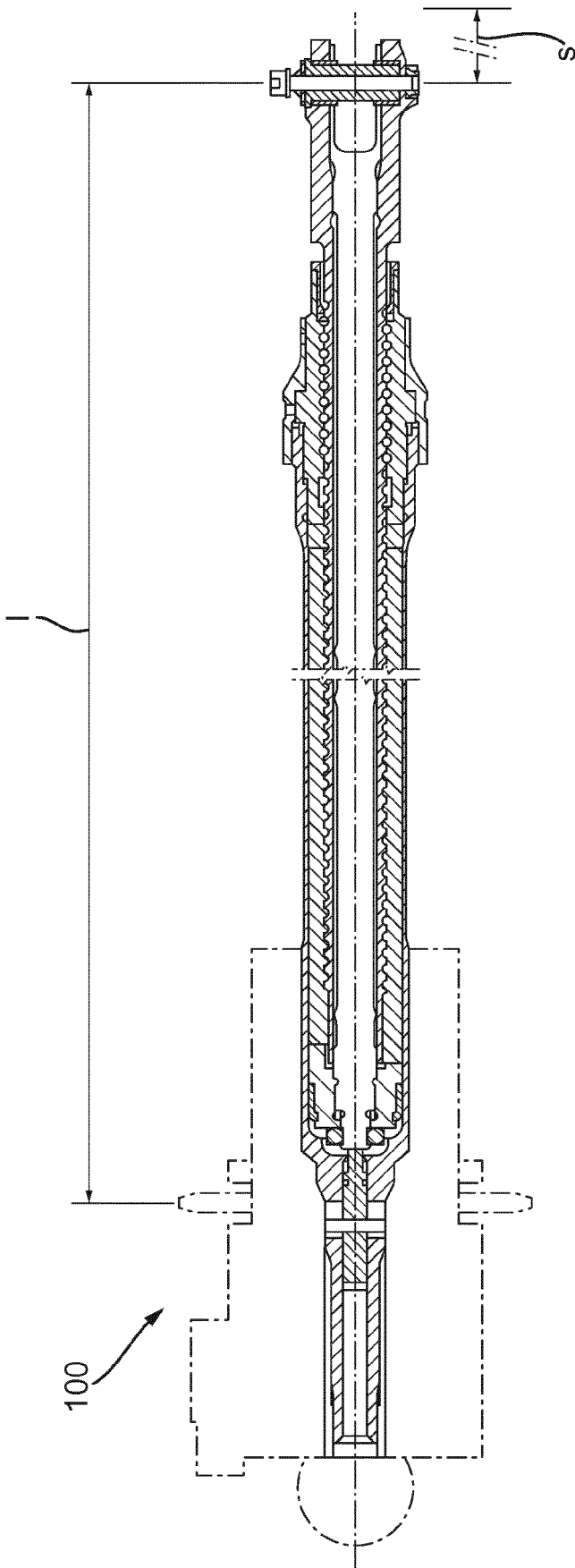
Fig. 3 Prior Art
