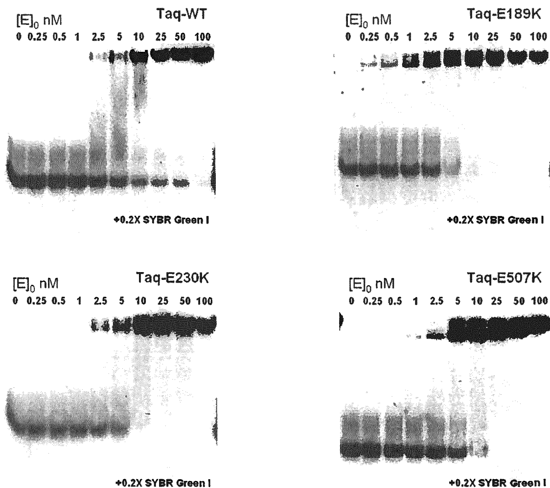
Figure 8. Polyacrylamid gel electrophoresis pictures of electrophoretic mobility shift assay (EMSA). Polymerase affinity to substrate (Kd) in the presence of 0.2X SYBR Green I dye was measured using radioactively labeled DNA substrate at 0.1 nM concentration and 0.25-100 nM protein concentration gradient.
