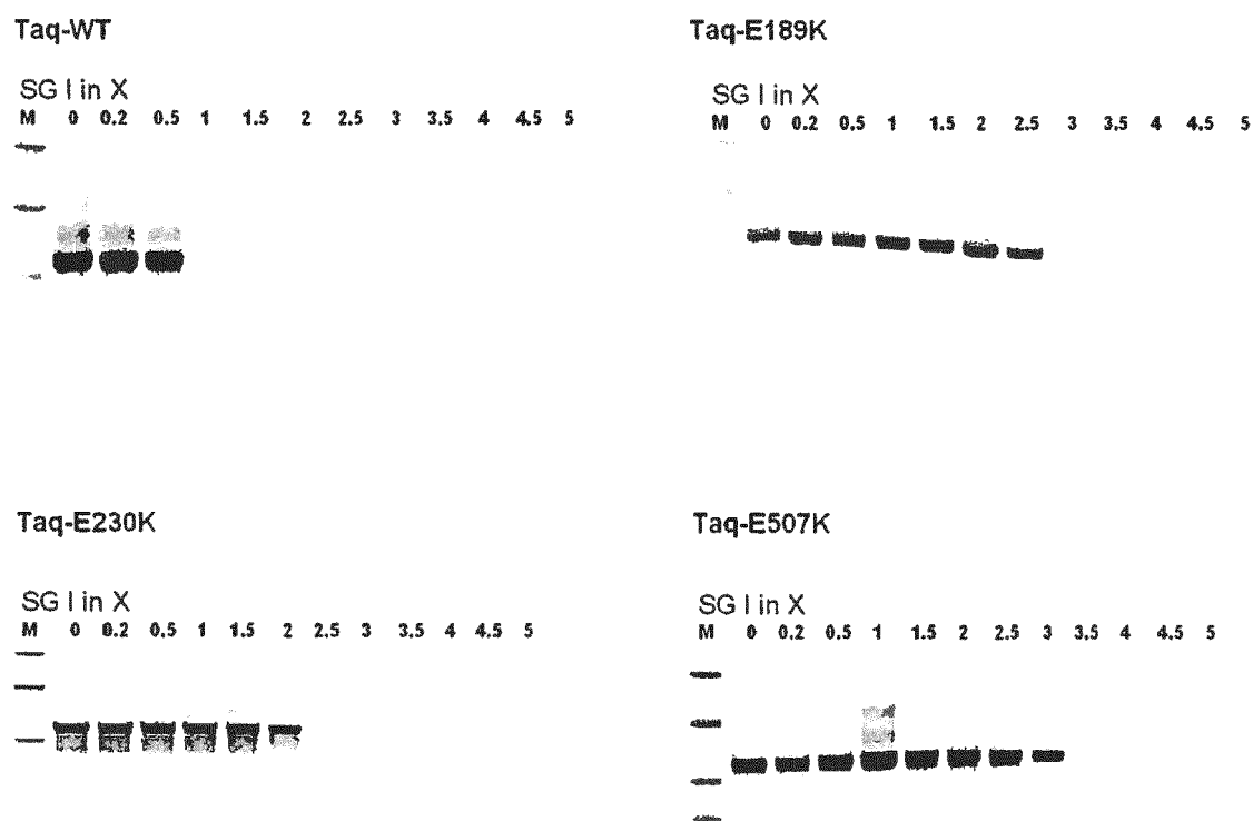
Figure 6. The PCR of 500 bp amplicon from human genomic DNA performed with wt His-Taq polymerase and single amino acid mutant polymerases at different SYBR Green I concentrations (SYBR Green I stock concentration is 10'000X and amplification was performed using 0.2-5X concentration of dye).
