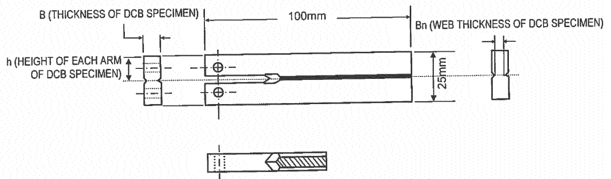
FIG. 1 NACE TM0177 method D DCB specimen
