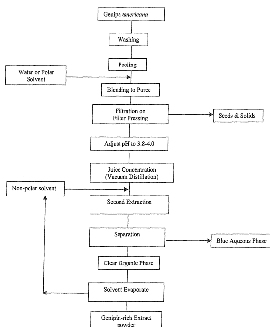
Figure 1 Process for Preparing Genipin-Rich Extract
