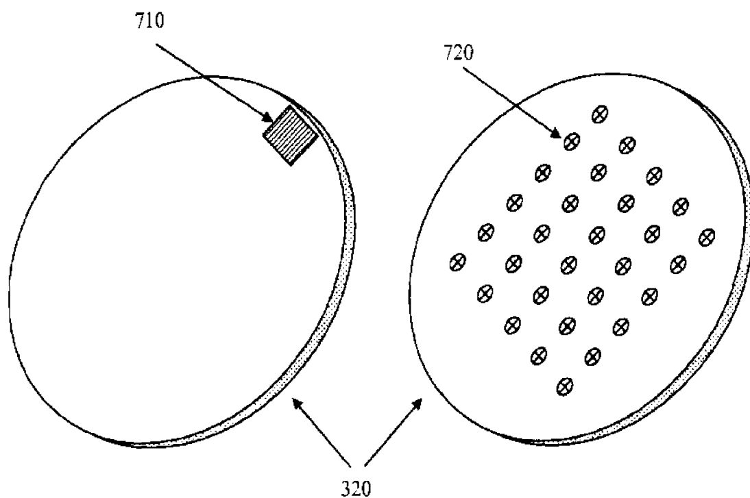
Figure 7 – A Schematic Diagram of Up (on right) and Down (on left) Sides of a Detachable Light Display Device with LEDs in a Computerized Yo-Yo
