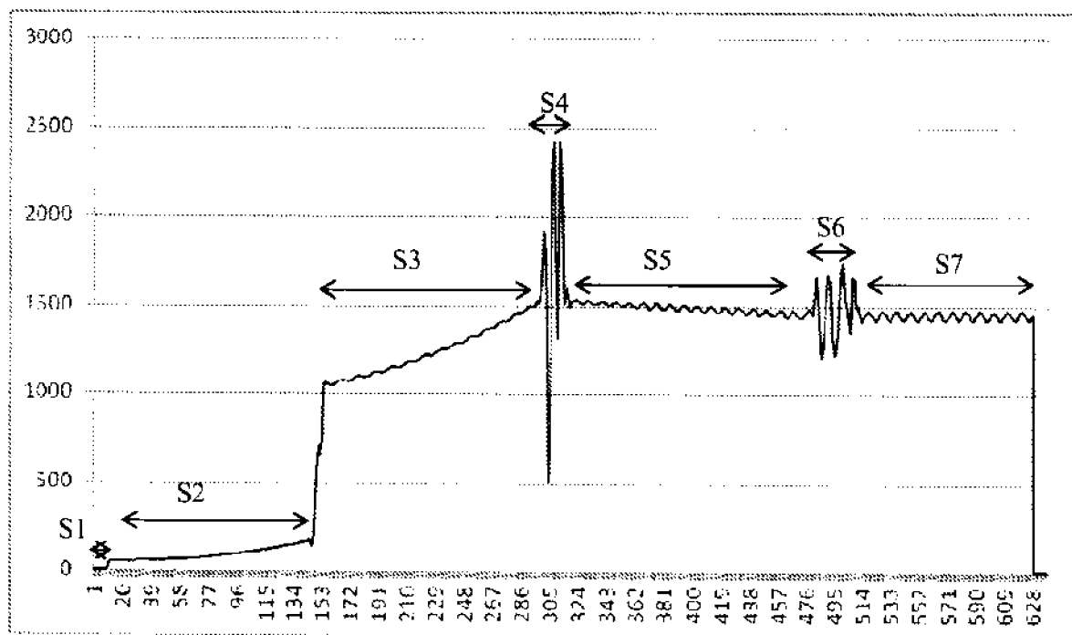
Figure 5 – An Example of an Acceleration Curve for a Yo-Yo Game Sequence
