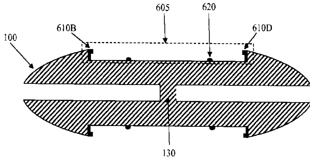
Figure 6B – A Schematic Side-View Cut of a Latching Base in a Computerized Yo-Yo
