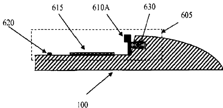
Figure 6C – A Side-View Cut of a Detail in a Latching Base in a Computerized Yo-Yo
