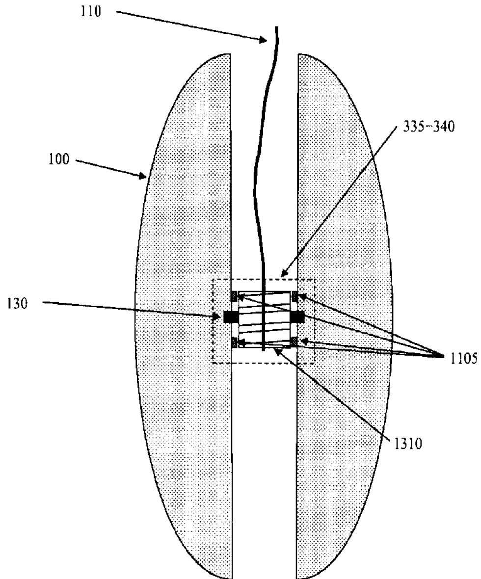
Figure 13 – A Schematic Side-View Diagram of an Electric Clutch Device and an Electric Motor Device in a Computerized Yo-Yo
