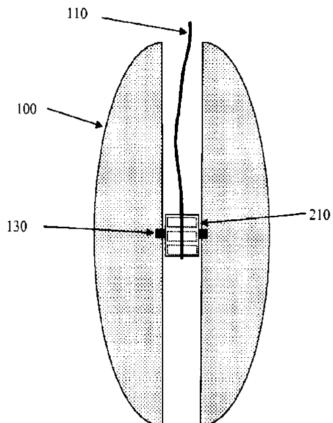
Figure 2 – A Schematic Side-View Diagram of a Ball Bearing Yo-Yo
