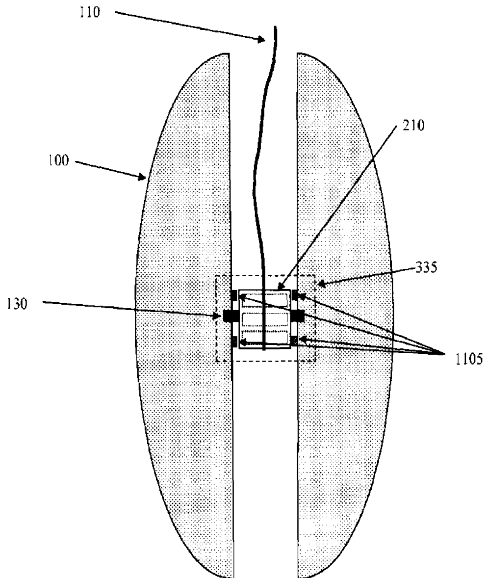
Figure 11 -- A Schematic Side-View Diagram of an Electric Clutch Device in a Computerized Yo-Yo
