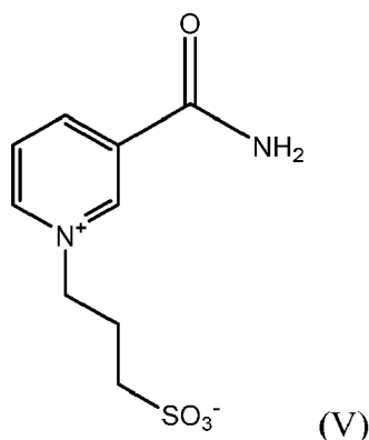
3-(3-carbamoylpyridin-1-ium-1-yl)propane-1-sulfonate
