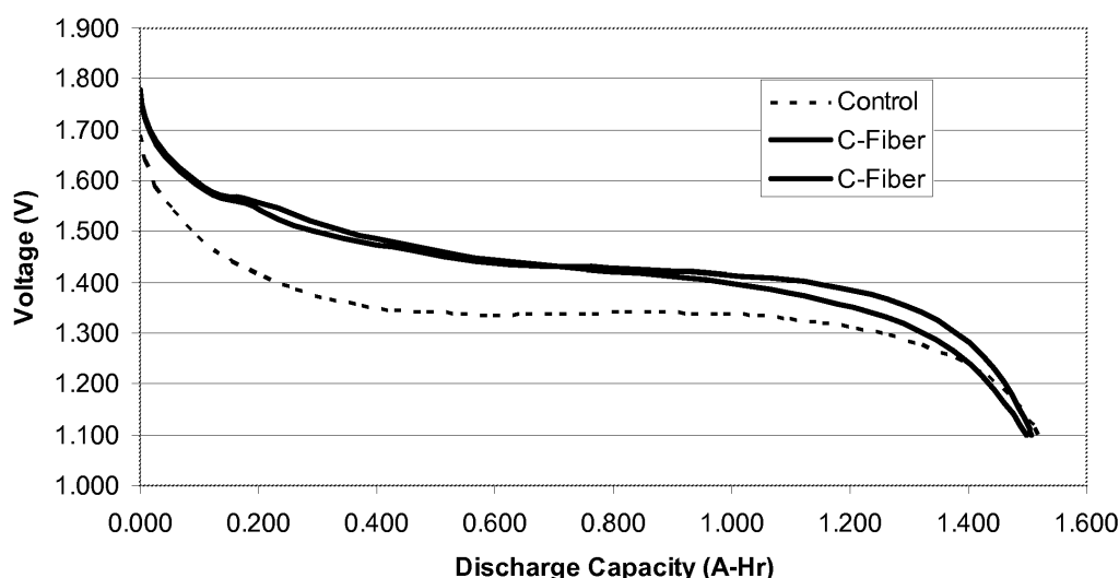
20Amp Discharge Curve at 152 Cycles
