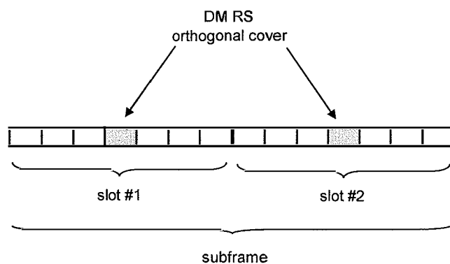
Fig. 6 Orthogonal cover applied for DM RS of MU-MIMO users
