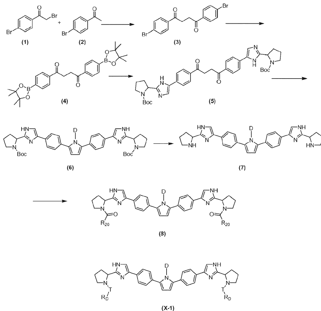
Scheme X
