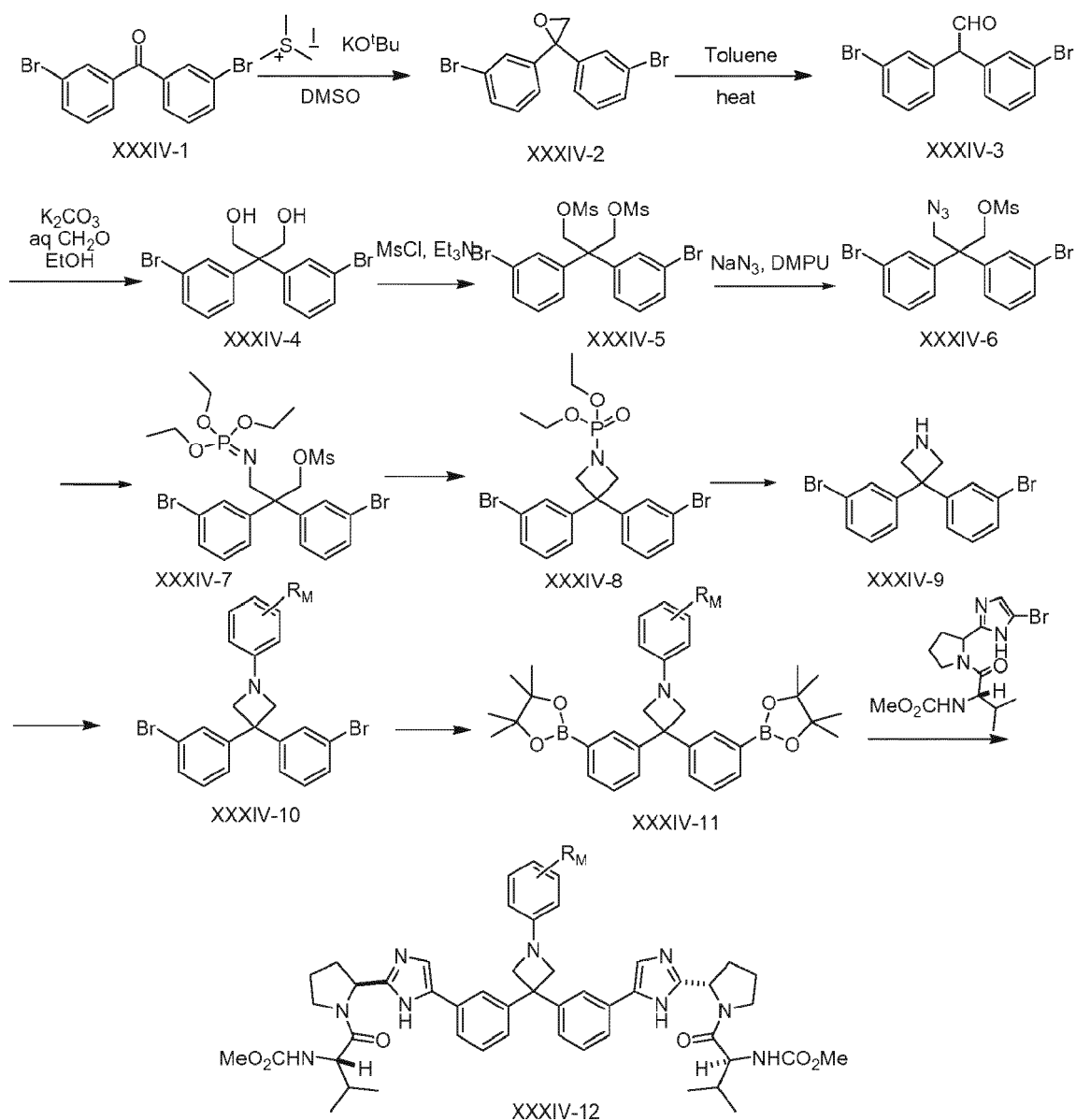
Scheme XXXIV
