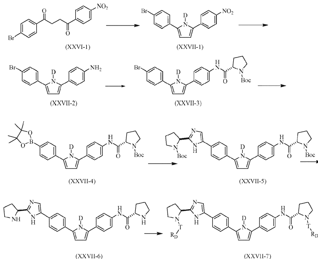
Scheme XXVII
