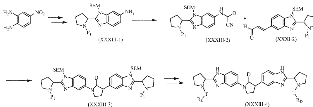
Scheme XXXIII
