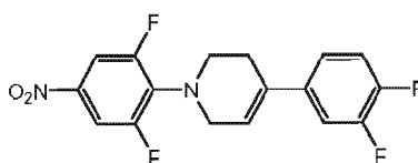
1-(2,6-difluoro-4-nitrophenyl)-4-(3,4-difluorophenyl)-1,2,3,6-tetrahydropyridine
