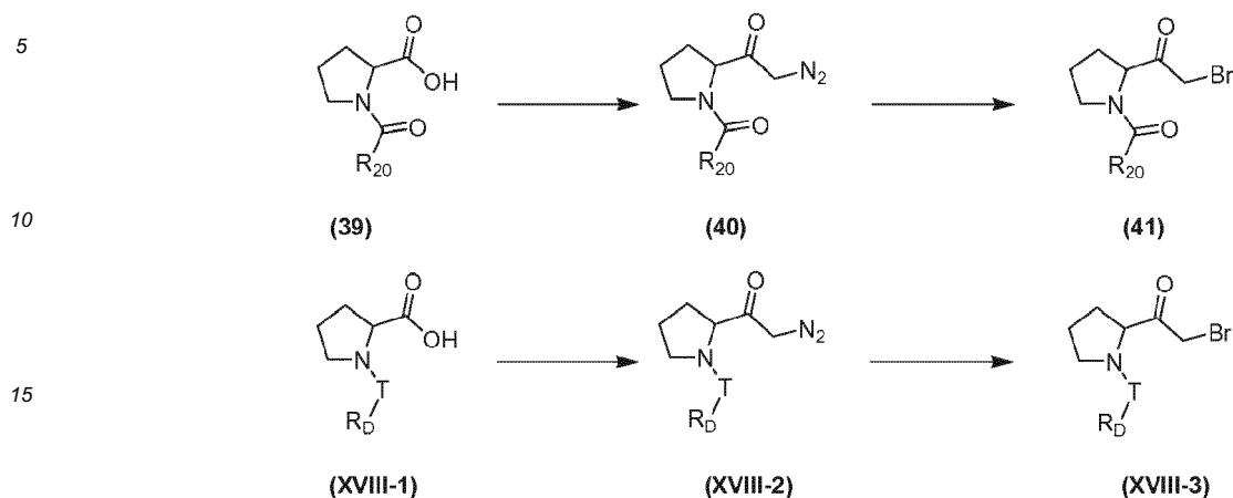
Scheme XVIII
