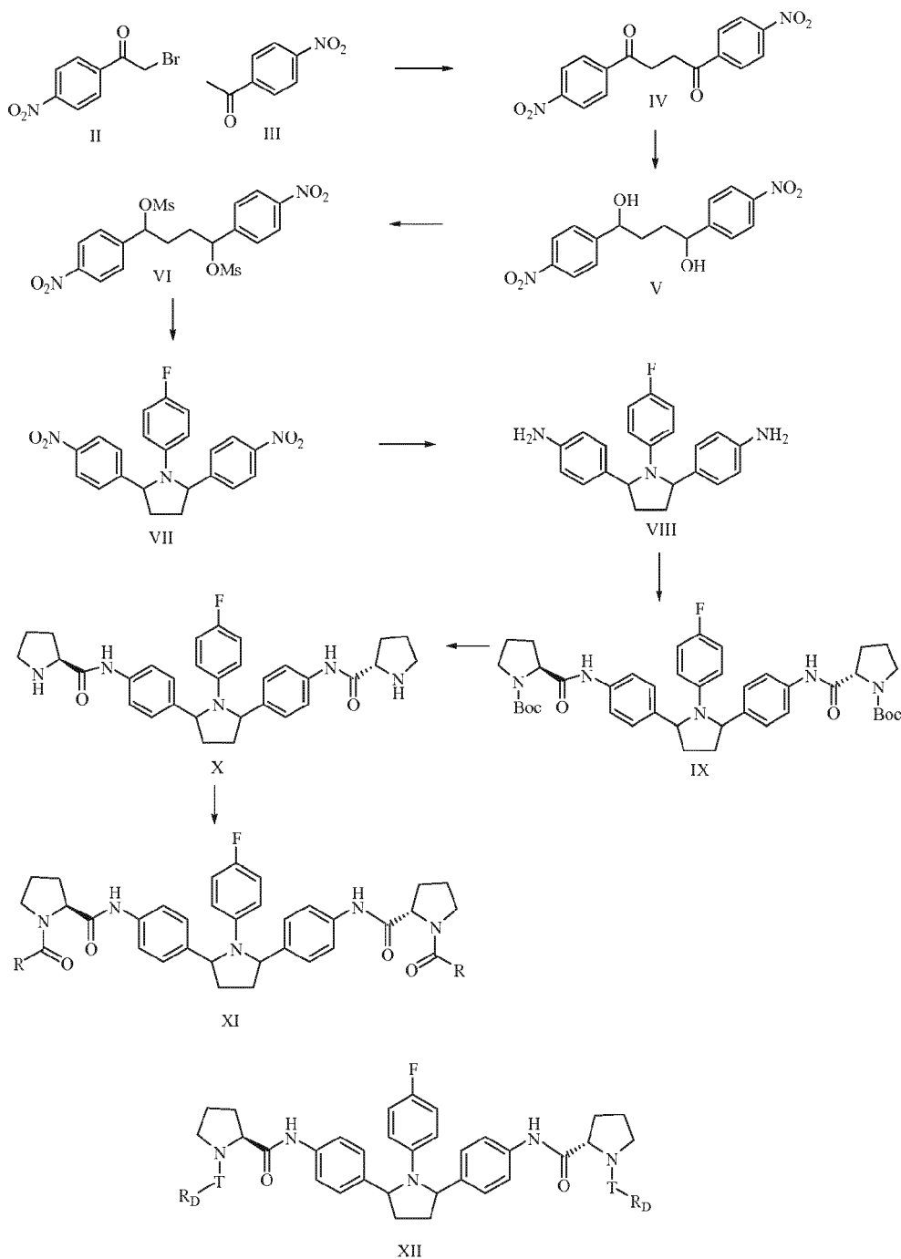
Scheme II
