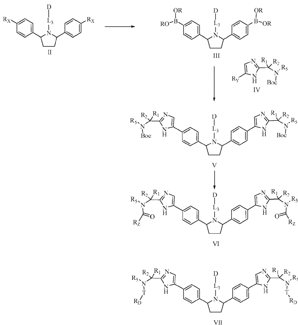
Scheme VII
