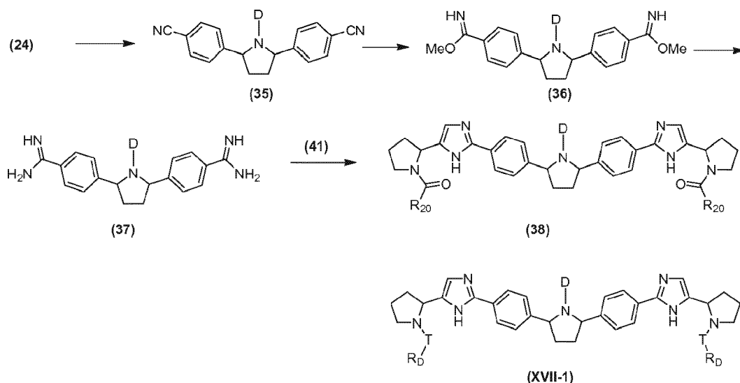
Scheme XVII
