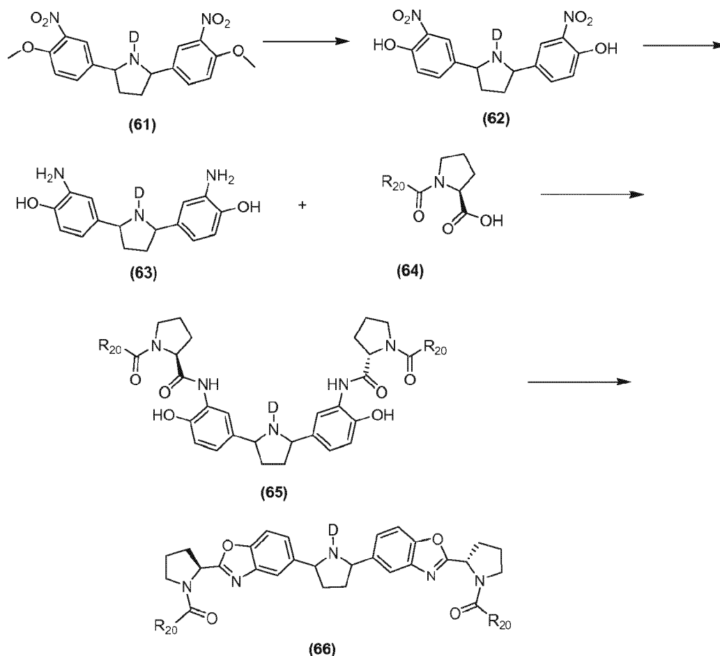
Scheme XXII
