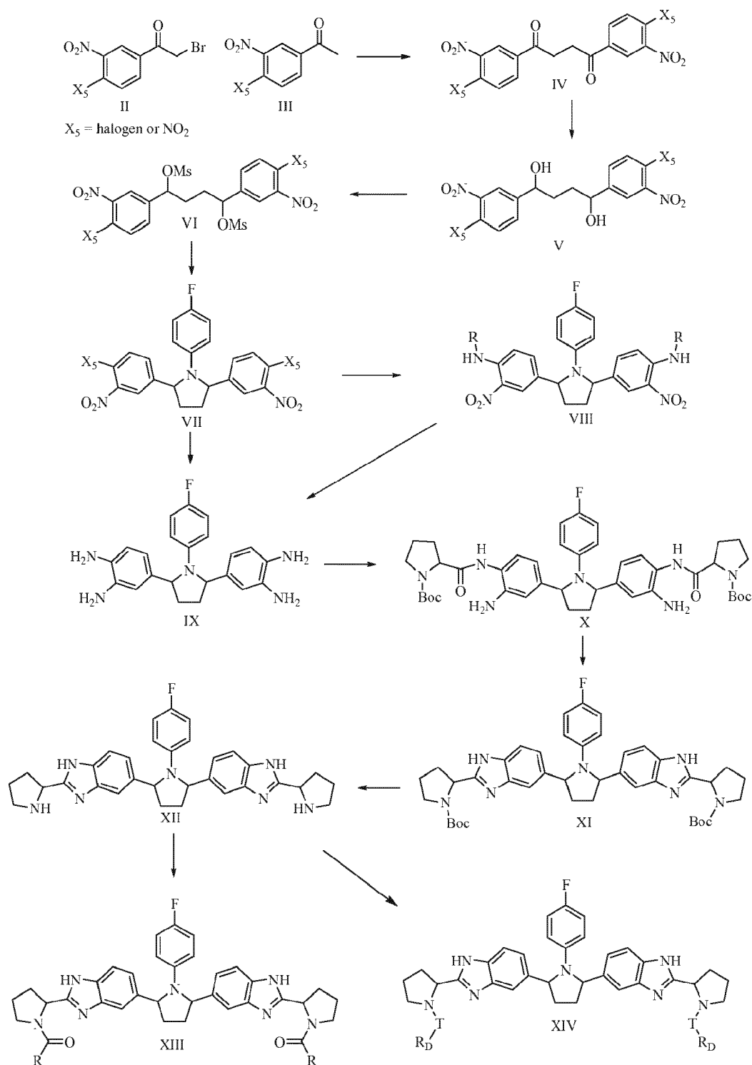
Scheme IV
