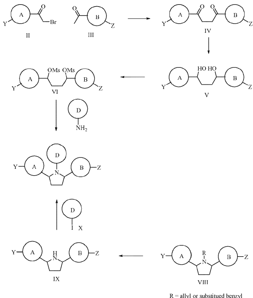
Scheme III
