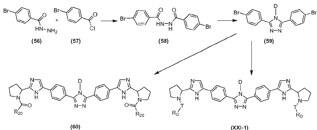
Scheme XXI
