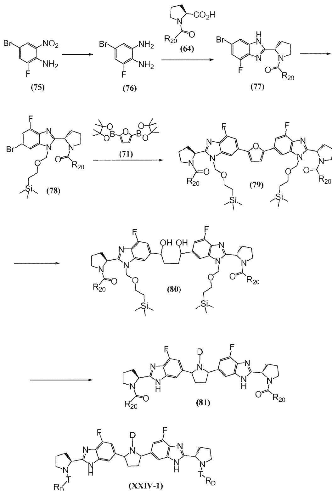
Scheme XXIV
