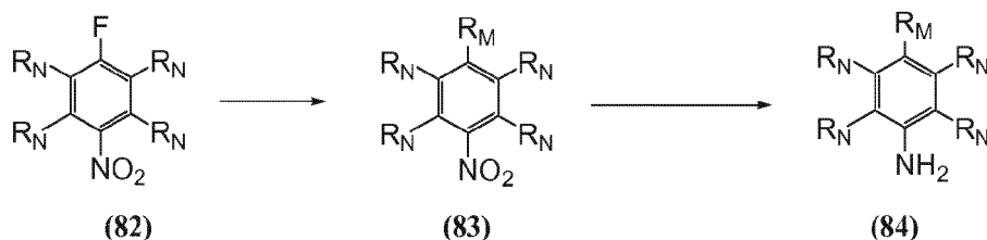
Scheme XXV
