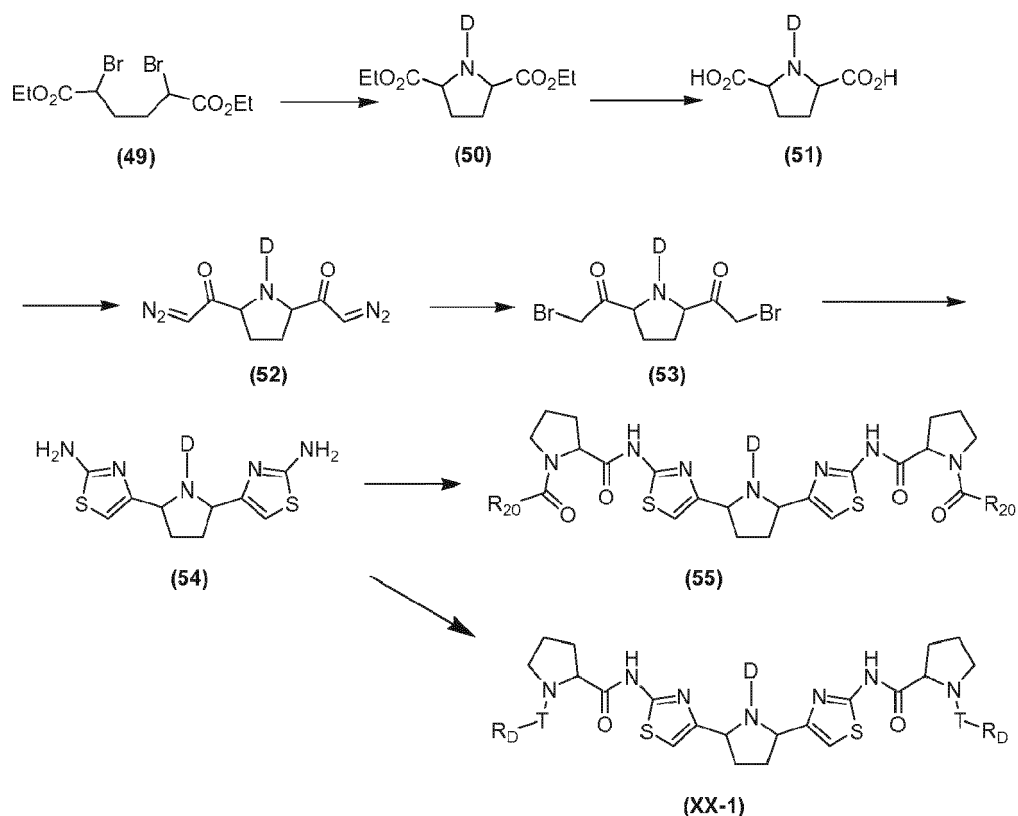
Scheme XX
