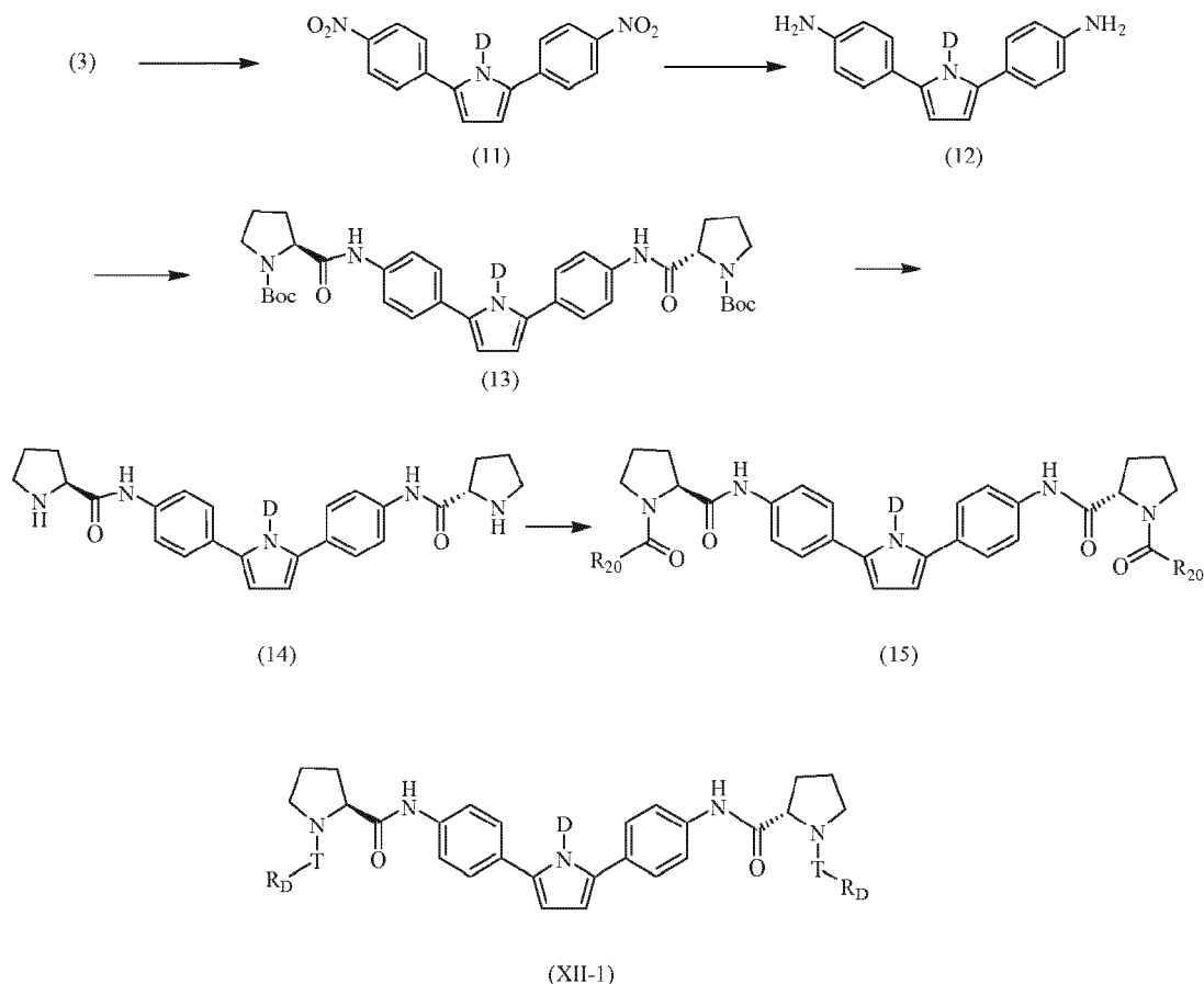
Scheme XII
