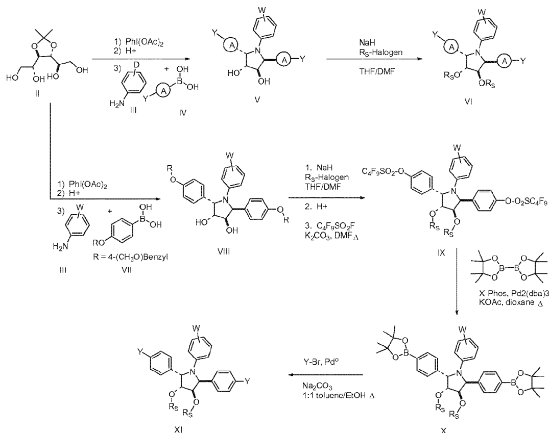
Scheme VIII
