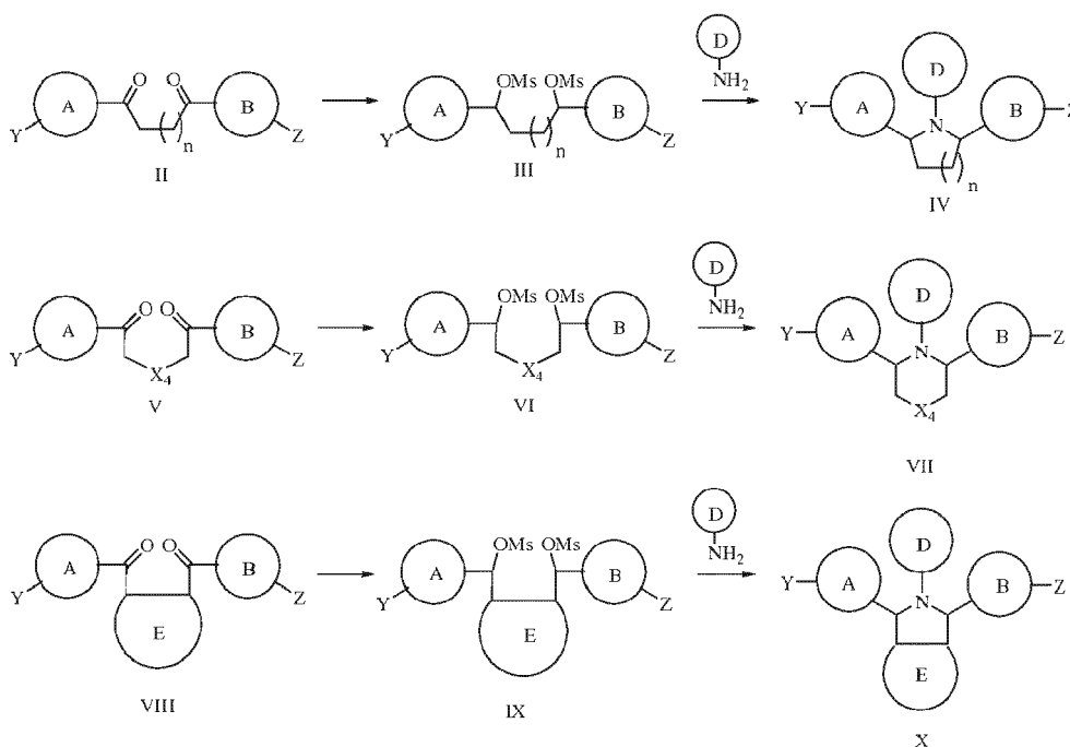
Scheme I
