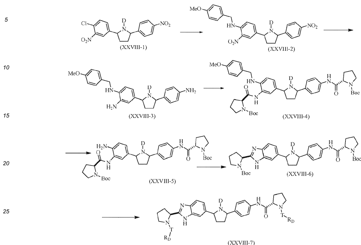
Scheme XXVIII
