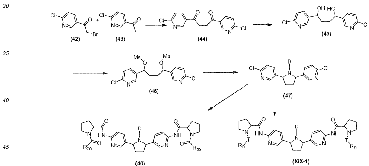
Scheme XIX
