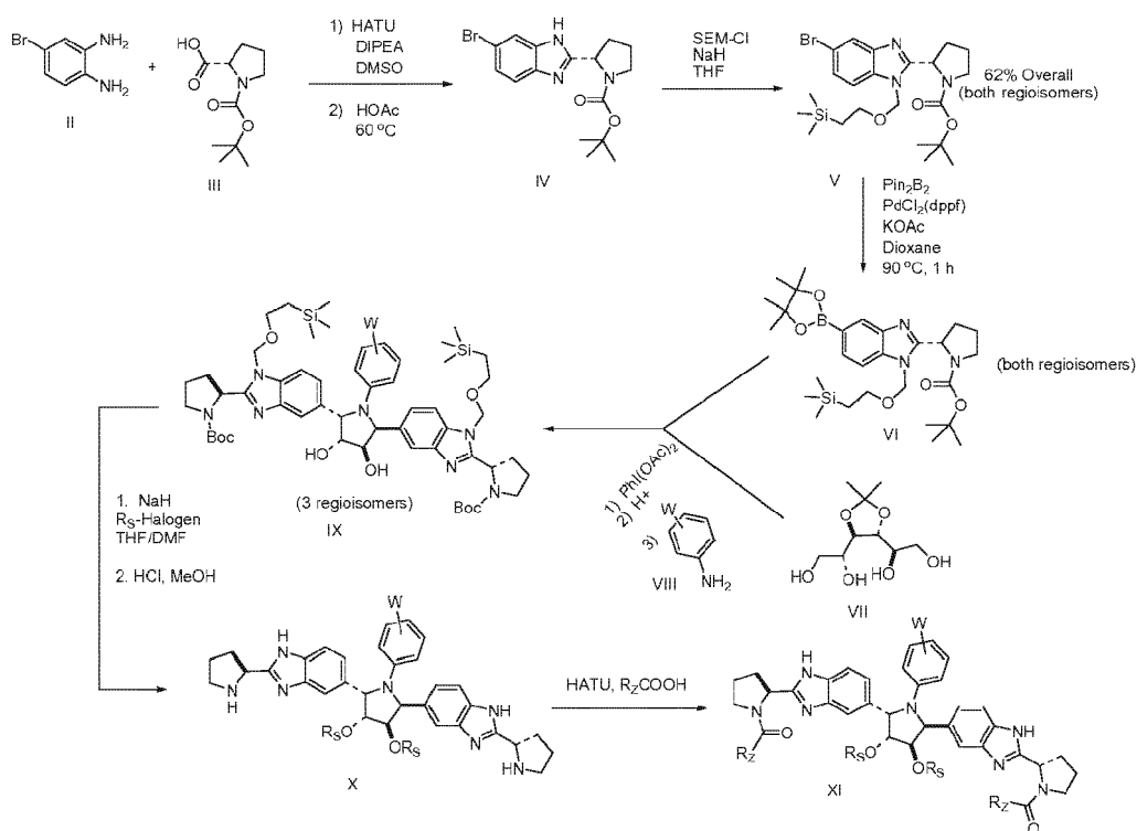
Scheme IX
