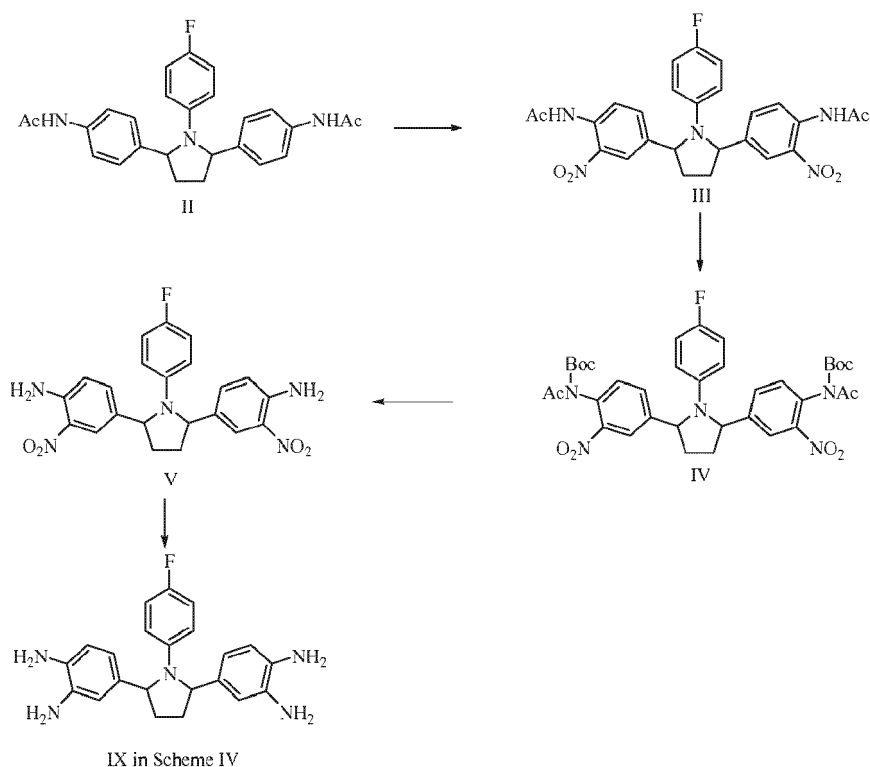
Scheme V
