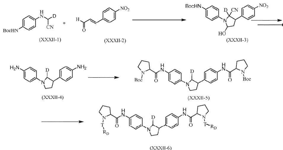
Scheme XXXII
