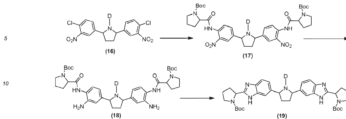
Scheme XIII
