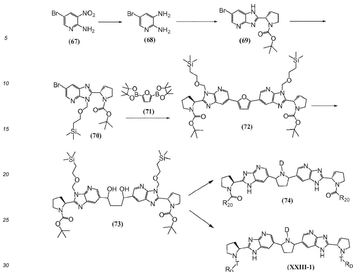
Scheme XXIII
