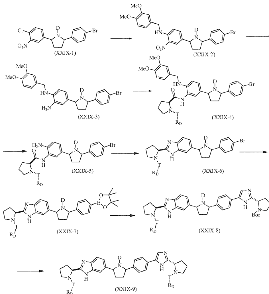
Scheme XXIX
