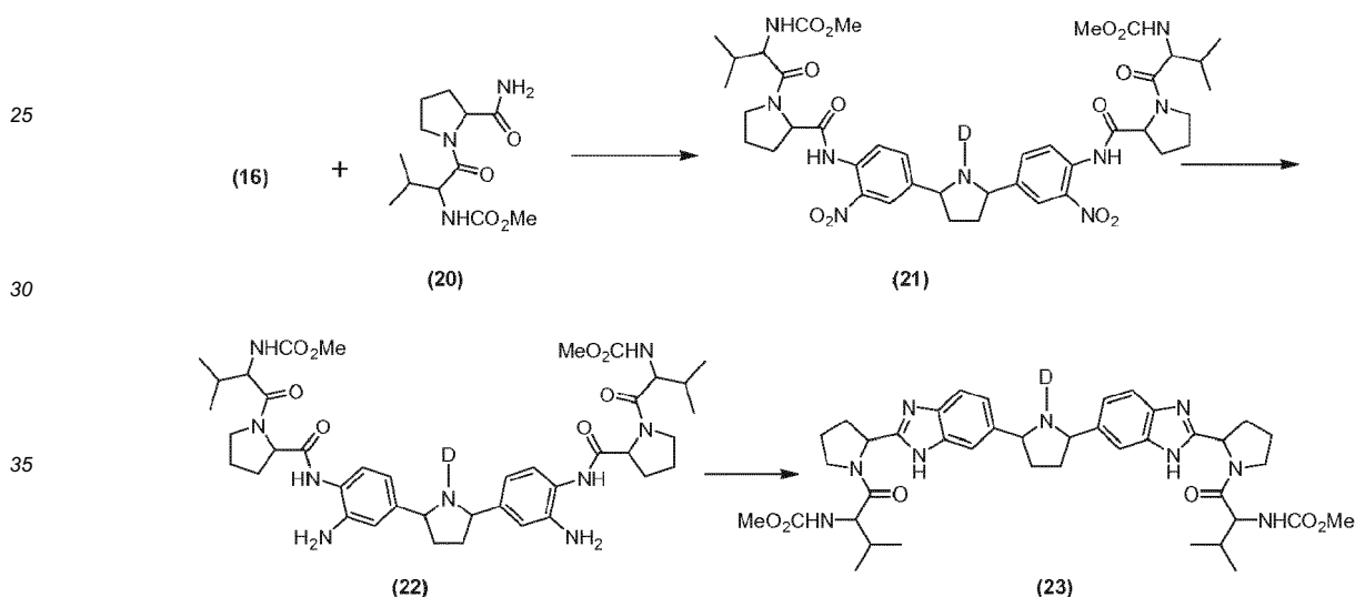
Scheme XIV
