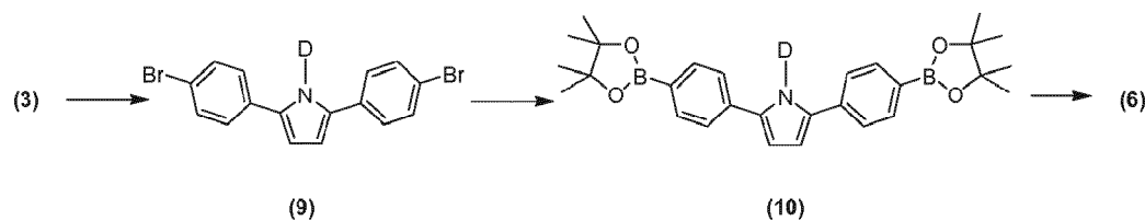
Scheme XI
