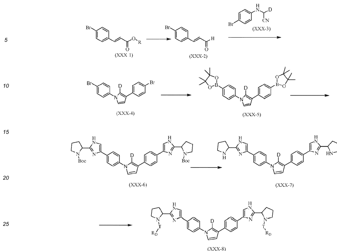
Scheme XXX
