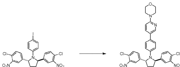
4-(5-(4-((2R,5R)-2,5-bis(4-chloro-3-nitrophenyl)pyrrolidin-1-yl)phenyl)pyridin-2-yl)morpholine
