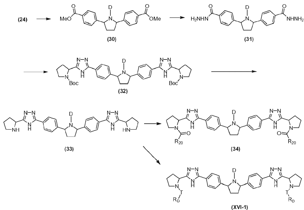
Scheme XVI
