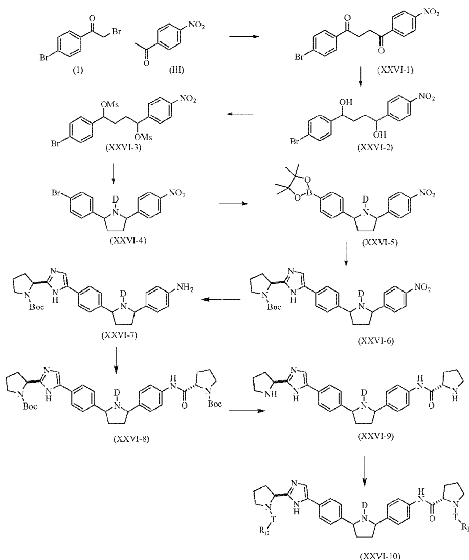
Scheme XXVI
