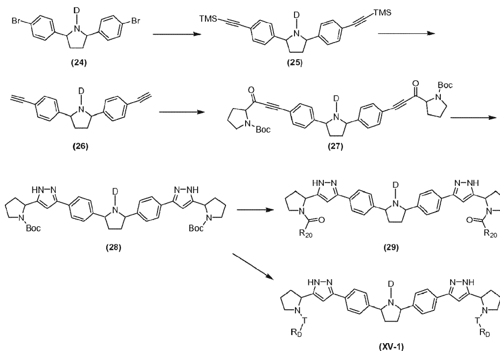
Scheme XV
