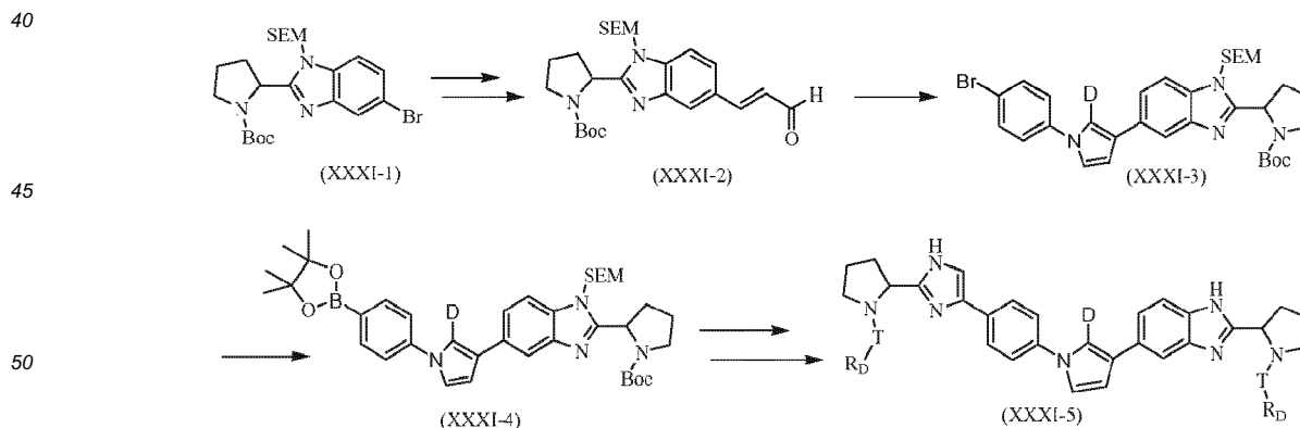
Scheme XXXI
