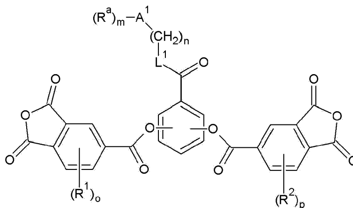
[Chemical Formula 1]
