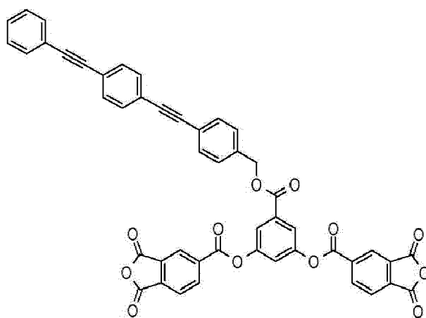
[Compound M-9]
