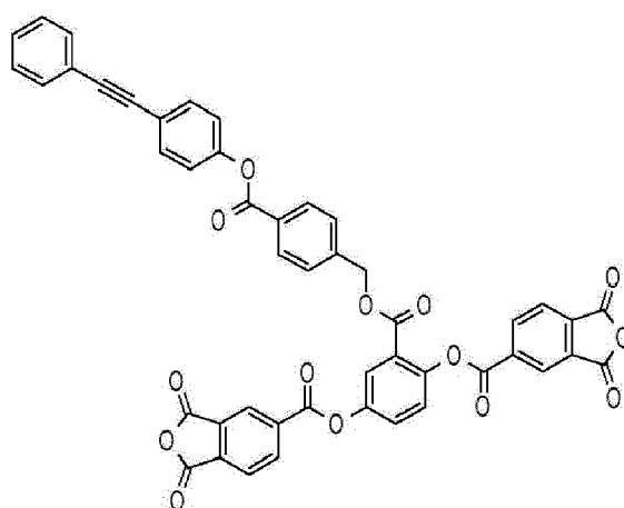
[Compound M-6]
