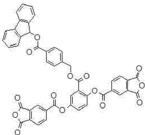
[Compound M-14]
