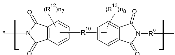
[Chemical Formula 18]
