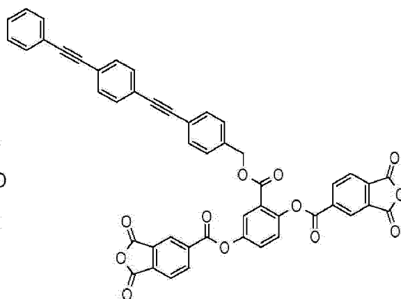
[Compound M-4]
