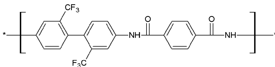
[Chemical Formula 22]
