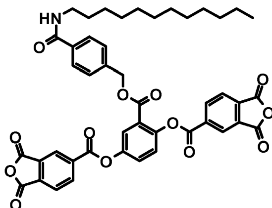
[Compound M-16]
