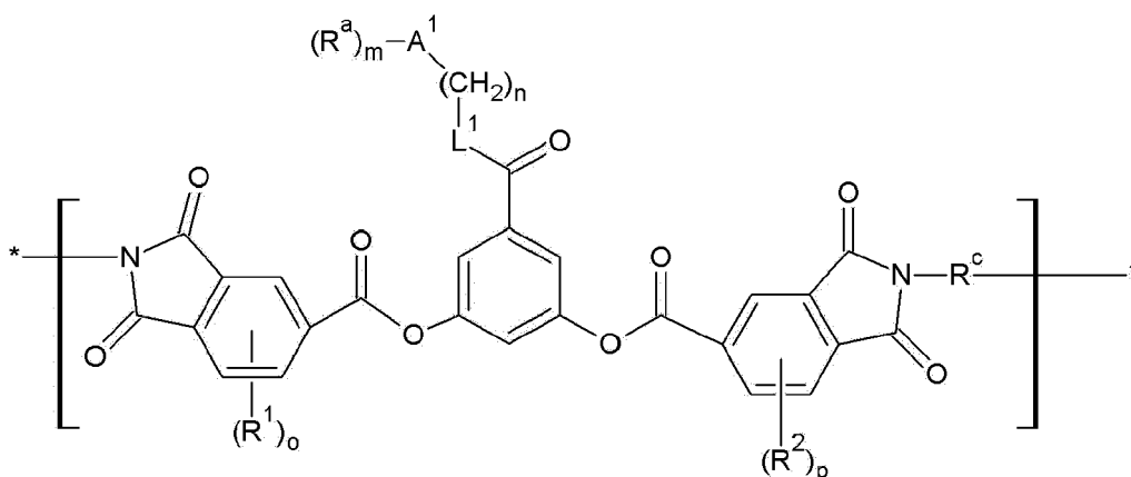
[Chemical Formula 15]
