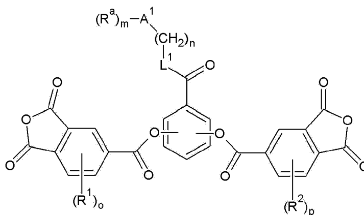
[Chemical Formula 1]
