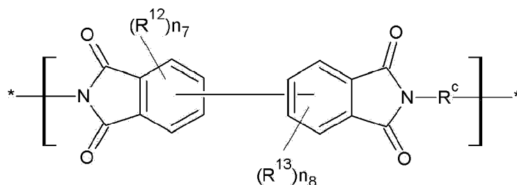
[Chemical Formula 20]
