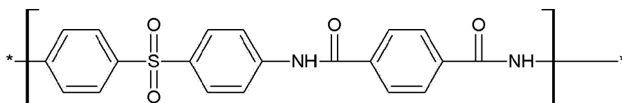
[Chemical Formula 23]
