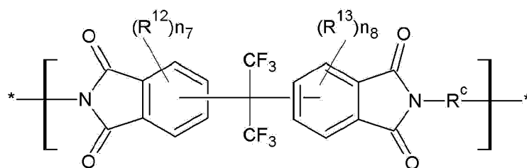
[Chemical Formula 20]
