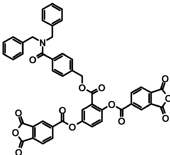
[Compound M-20]
