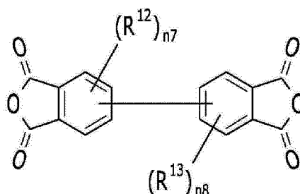
[Chemical Formula 11]
