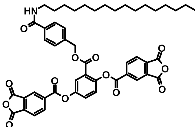
[Compound M-17]
