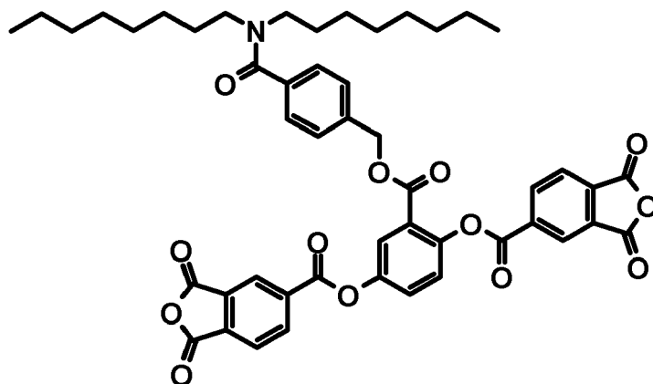
[Compound M-20]
