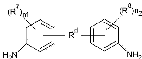
[Chemical Formula 6]
