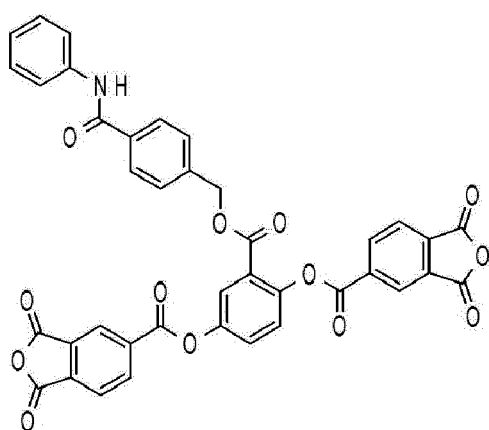
[Compound M-5]
