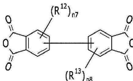
[Chemical Formula 11]
