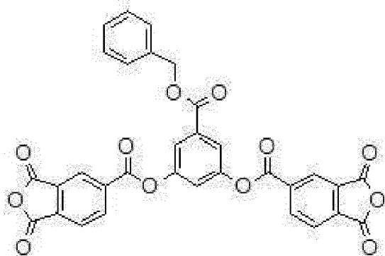
[Compound M-12]
