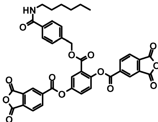
[Compound M-14]
