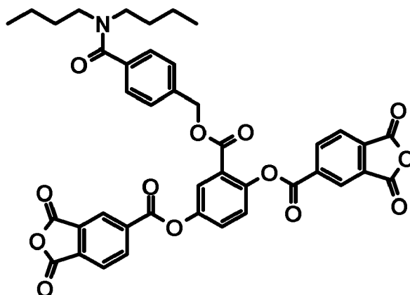
[Compound M-19]
