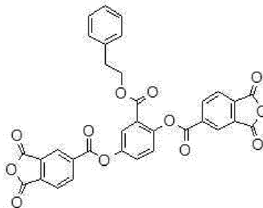
[Compound M-13]
