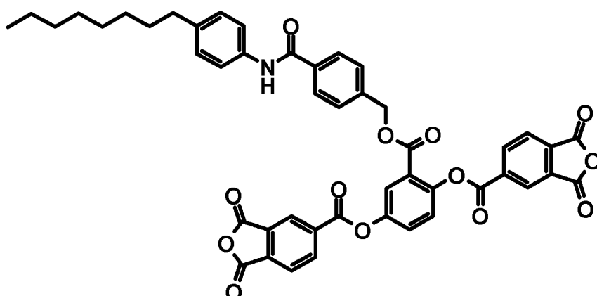
[Compound M-17]
