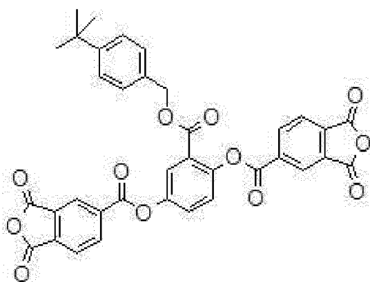
[Compound M-8]
