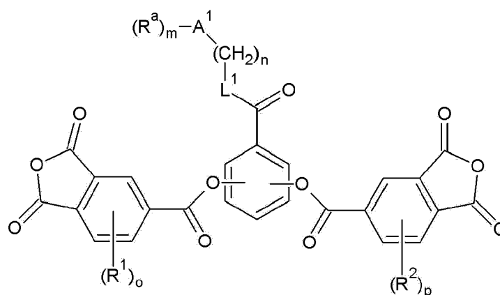
[Chemical Formula 1]
