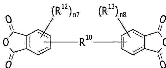
[Chemical Formula 9]
