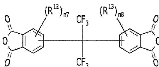
[Chemical Formula 11]
