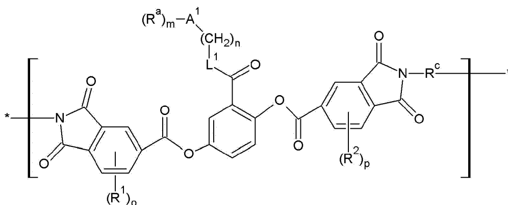
[Chemical Formula 14]
