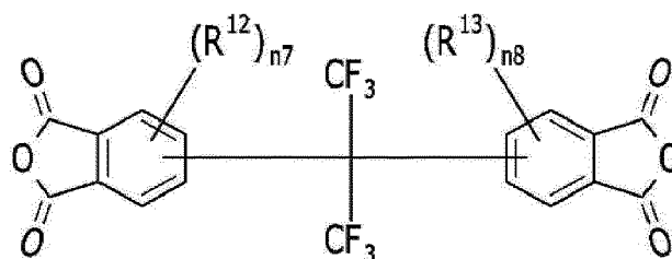
[Chemical Formula 11]
