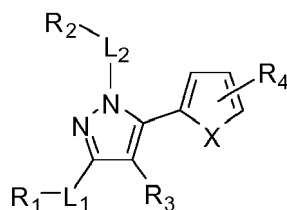
Formula (IV);
