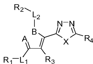
55 Formula (A);
