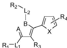
Formula (F);
