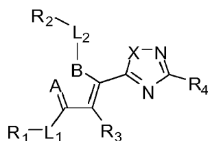
Formula (B);
