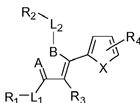
Formula (F);
