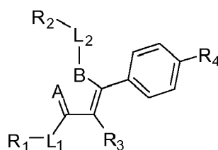
Formula (E);
