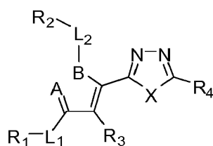
Formula (A);
