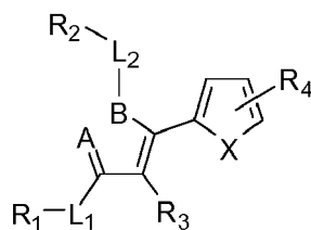
Formula (F);
