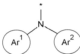
[Chemical Formula 2A]
