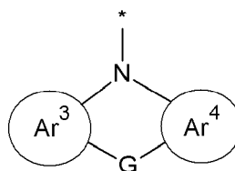
[Chemical Formula 2B]
