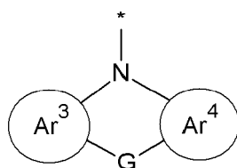
[Chemical Formula 2B]
