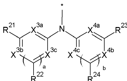
[Chemical Formula 2A-1]
