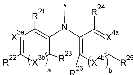
[Chemical Formula 2B-1]
