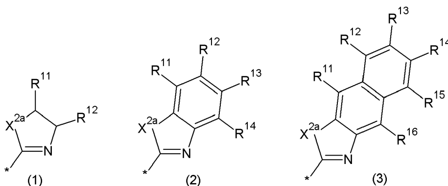
[Chemical Formula 3A]
