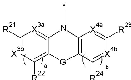
[Chemical Formula 2B-2]
