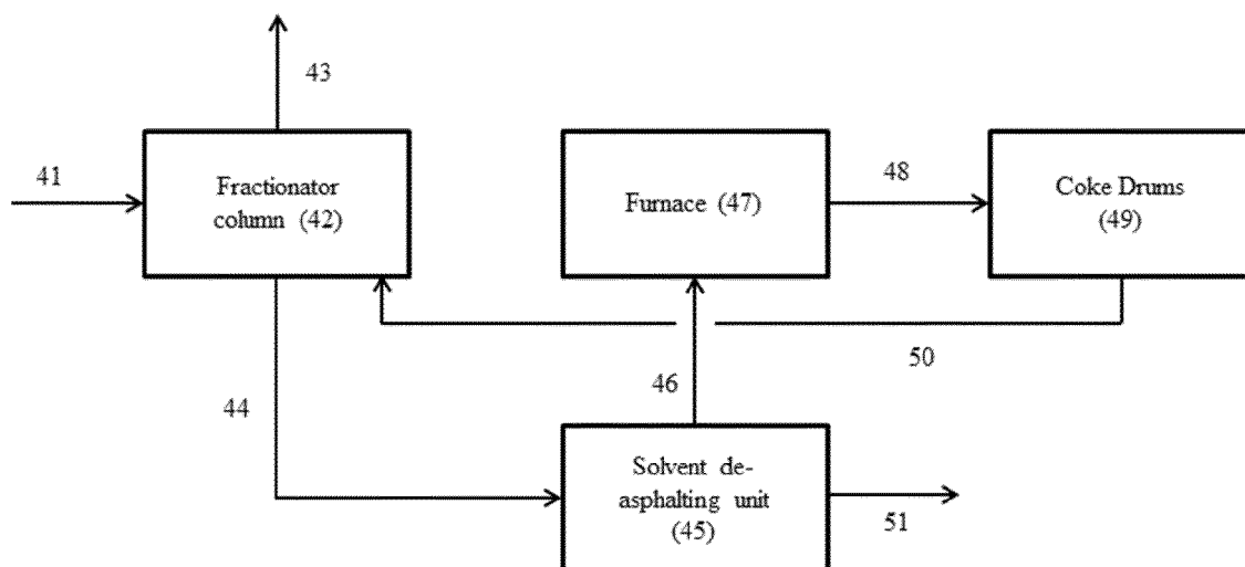
Fig. 3 Schematic diagram of process of present invention
