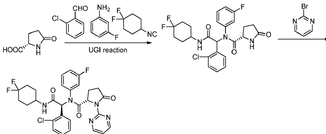
Compound 4
