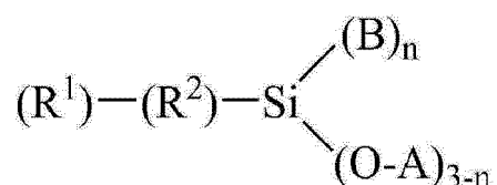
[Chemical Formula 14]
