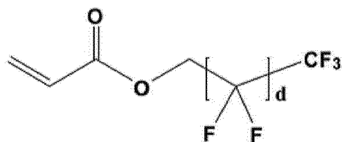
[Chemical Formula 3]
