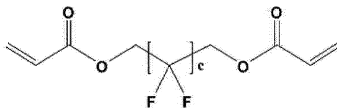
[Chemical Formula 2]
