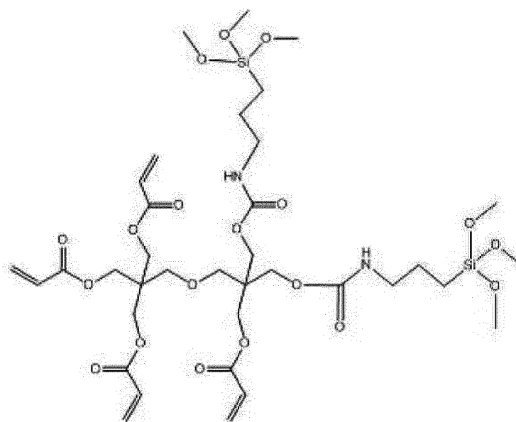
[Chemical Formula 14]
