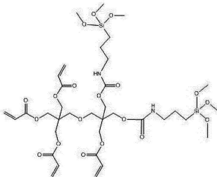
[Chemical Formula 14]
