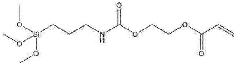
[Chemical Formula 12]
