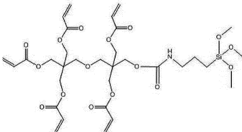
[Chemical Formula 13]
