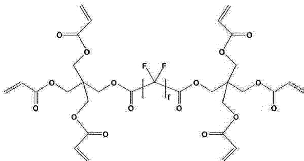
[Chemical Formula 5]
