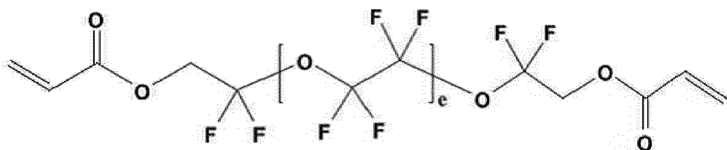
[Chemical Formula 4]
