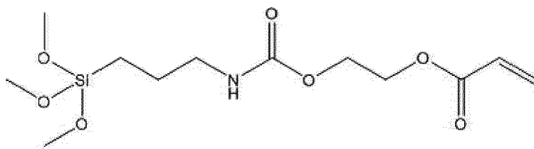
[Chemical Formula 12]
