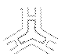
Two nick
