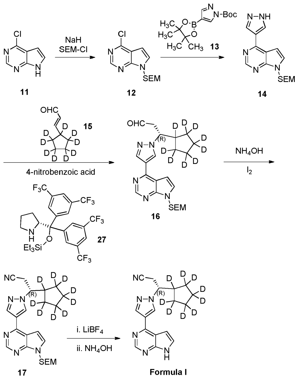
Scheme 1. Preparation of a Compound of Formula I.
