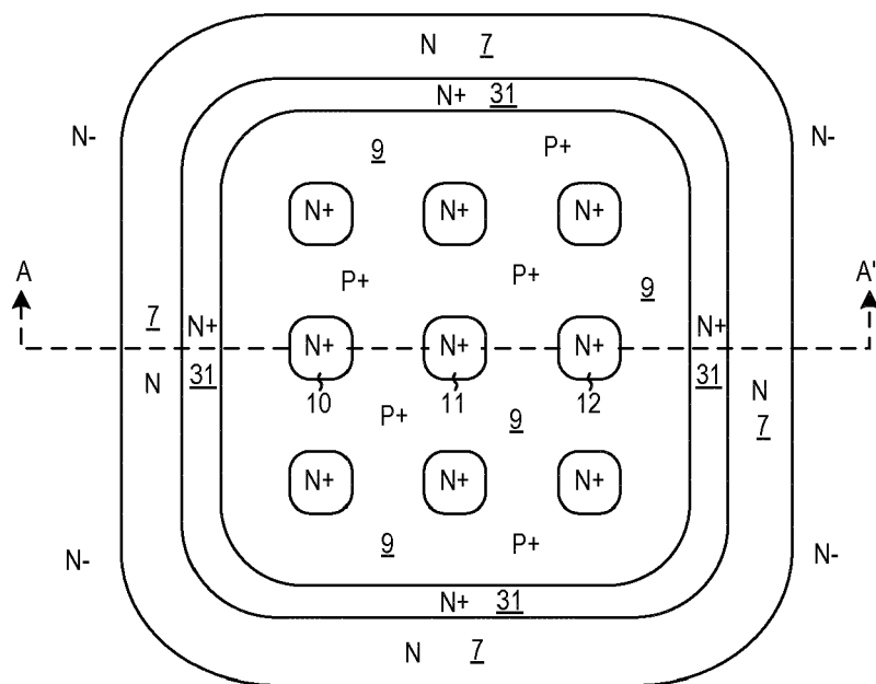
TOP-DOWN VIEW OF THE SEMICONDUCTOR SURFACE
