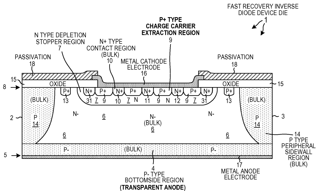
FAST RECOVERY INVERSE DIODE
