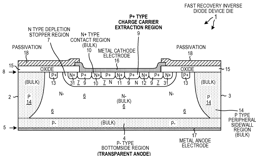
FAST RECOVERY INVERSE DIODE FIG. 1
