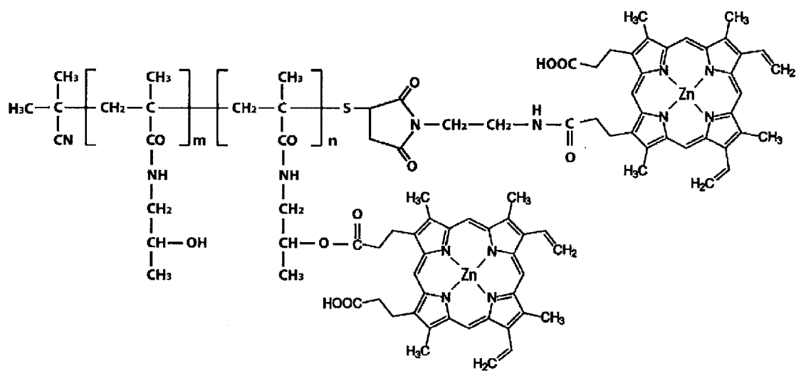
(5) Poly-HPMA-ZnPP
