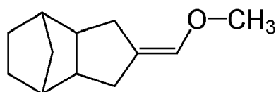
1-(Ethoxymethylene)octahydro-1 H -4,7-methanoindene (Structure 3)
