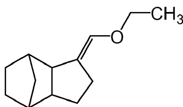
2-(Ethoxymethylene)octahydro-1 H -4,7-methanoindene (Structure 4)
