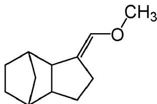
2-(Methoxymethylene)octahydro-1 H -4,7-methanoindene (Structure 2)
