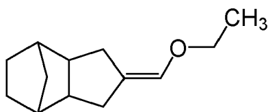
2-(Ethoxymethylene)octahydro-1 H -4,7-methanoindene (Structure 4)
