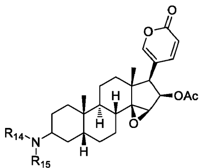
Formula If
