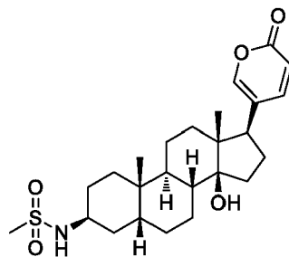
N-((3S,5R,8R,9S,10S,13R,14S,17R)-14-hydroxy-10,13-dimethyl-17-(2-oxo-2H-pyran-5-yl)hexadecahydro-1H-cyclopenta[a]phenanthren-3-yl)methanesulfonamide
