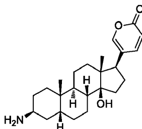
5-((3S,5R,8R,9S,10S,13R,14S,17R)-3-amino-14-hydroxy-10,13-dimethylhexadecahydro-1H-cyclopenta[a]phenanthren-17-yl)-2H-pyran-2-one
