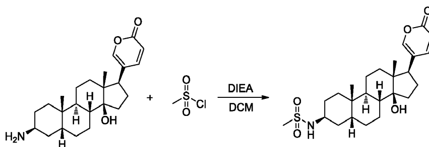
N-((3S,5R,8R,9S,10S,13R,14S,17R)-14-hydroxy-10,13-dimethyl-17-(2-oxo-2H-pyran-5-yl)hexadecahydro-1H-cyclopenta[a]phenanthren-3-yl)methanesulfonamide
