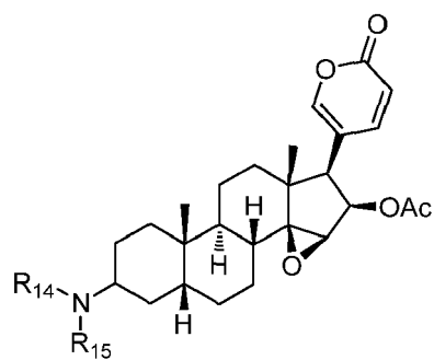
Formula If
