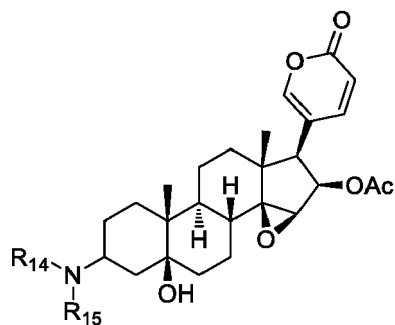
Formula Ig
