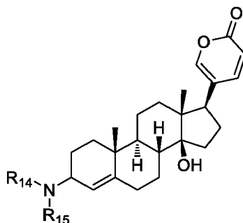
Formula Id
