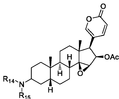
Formula If
