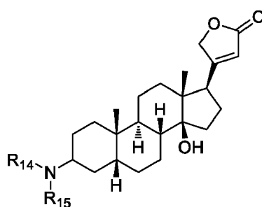
Formula Ih
