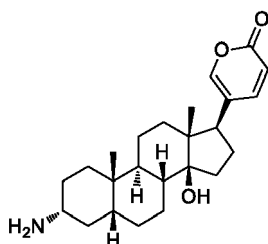
5-((3R,5R,8R,9S,10S,13R,14S,17R)-3-amino-14-hydroxy-10,13-dimethylhexadecahydro-1H-cyclopenta[a]phenanthren-17-yl)-2H-pyran-2-one
