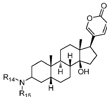
Formula Ia
