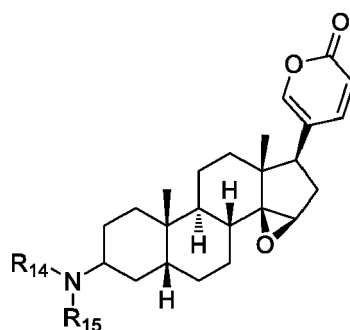
Formula Ie
