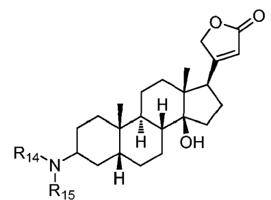
Formula Ih
