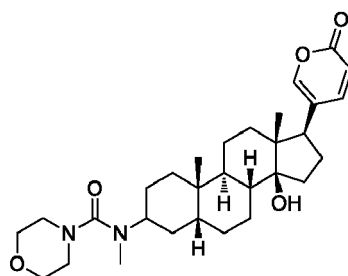
N-((5R,8R,9S,10S,13R,14S,17R)-14-hydroxy-10,13-dimethyl-17-(2-oxo-2H-pyran-5-yl)hexadecahydro-1H-cyclopenta[a]phenanthren-3-yl)-N-methylmorpholine-4-carboxamide
