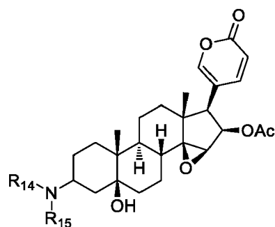
Formula Ig
