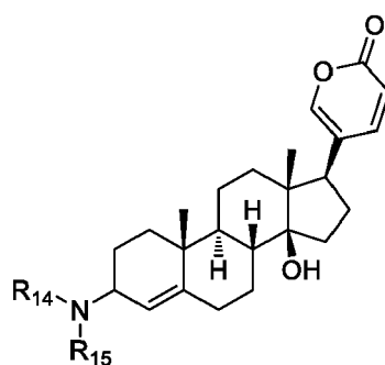
Formula Id
