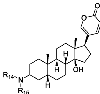
Formula Ia
