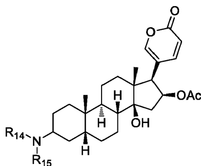
Formula Ib
