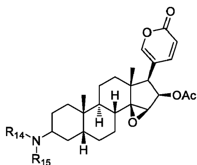
Formula If
