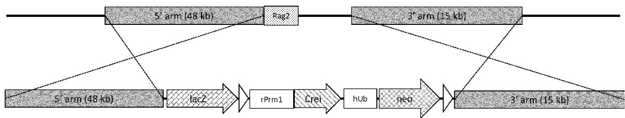
Rat Rag2 Locus and Large Targeting Vector
