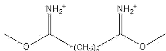
[Chemical Formula 1]
