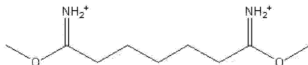
[Chemical Formula 3]
