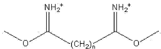
[Chemical Formula 1]
