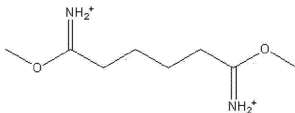
[Chemical Formula 4]
