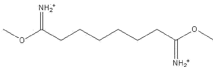
[Chemical Formula 4]
