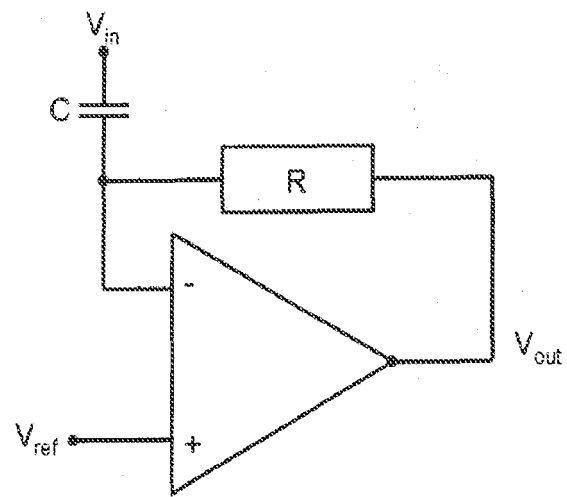
Differentiator circuit with clamped capacitor ( V_c clamped to V_{ref} )
