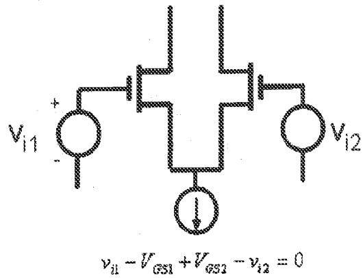
Differential Amplifier for Trigger Circuit
