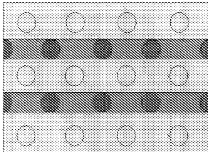
Top view of photonic and fluidic ports on top half of durable ATE socket
