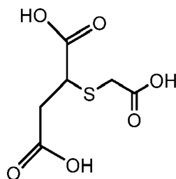
(III) 2-(carboxymethylthio) succinic acid.
