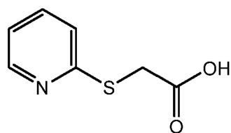
(II) (2-pyridinylsulfanyl)-acetic acid; and,
