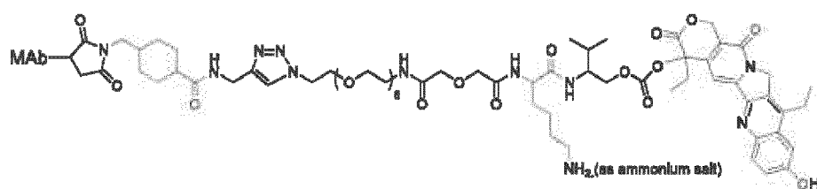
MAb-CL7-SN-38,
