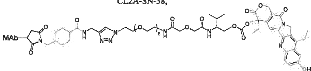
CL2A-SN-38,
