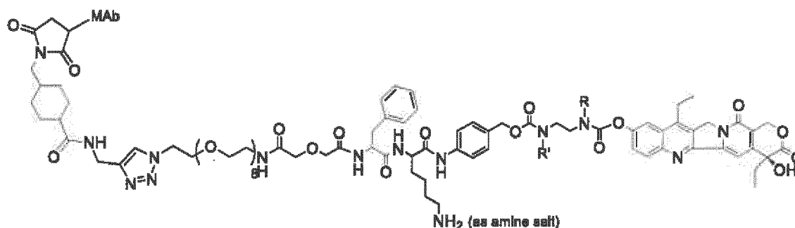
MAb-CLY-SN-38,
