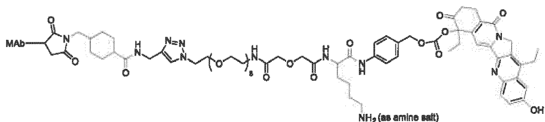
CL2A-SN-38,
