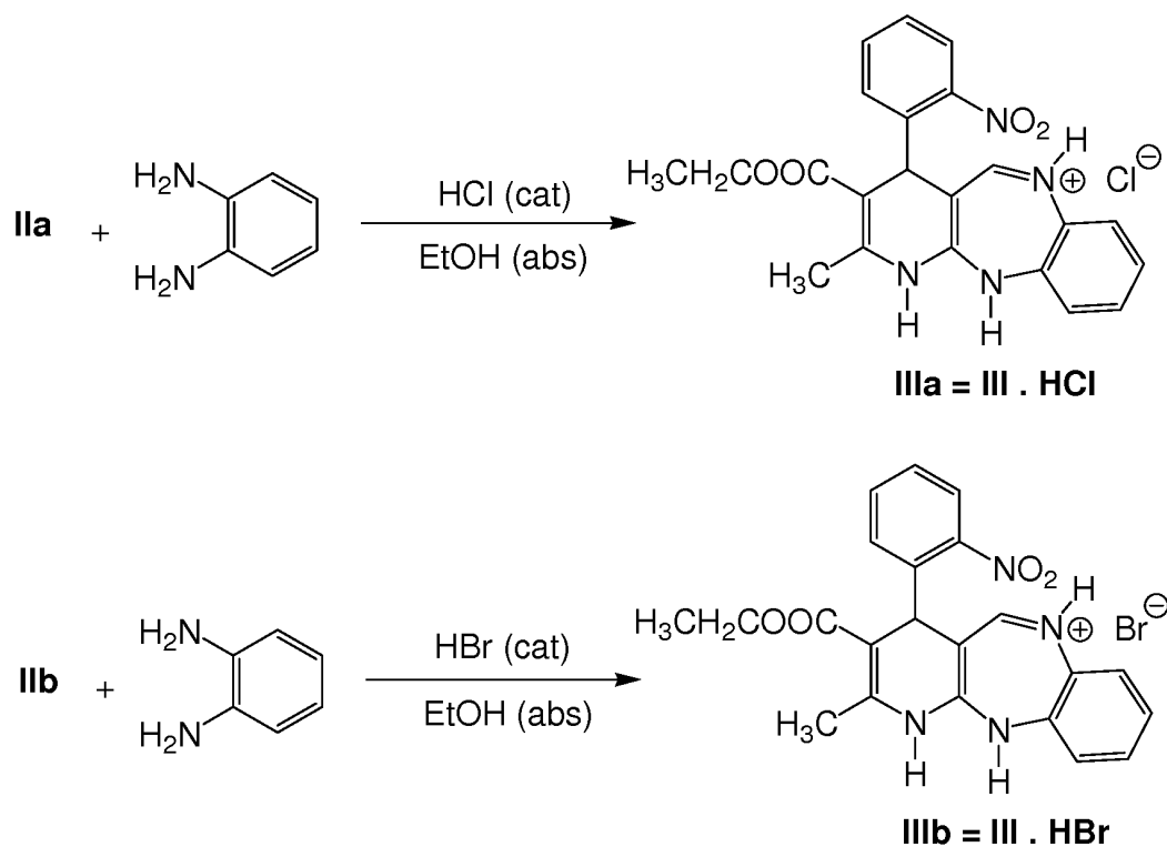
Scheme for obtaining Compound III and its Halohydrates
