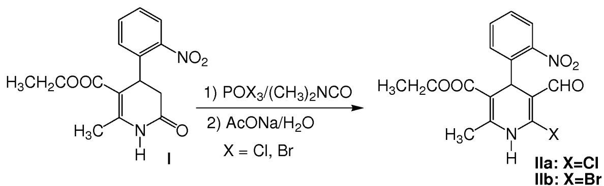
Scheme for obtaining IIa and IIb
