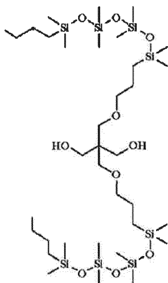
Silicon-containing compound-4
