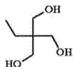
Hydroxy compound-2
