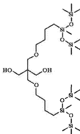
Silicon-containing compound-5
