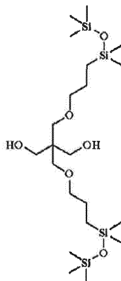
Silicon-containing compound-2
