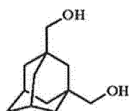
Hydroxy compound-1
