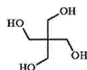
Hydroxy compound-3
