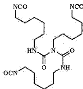
Isocyanate compound-5
