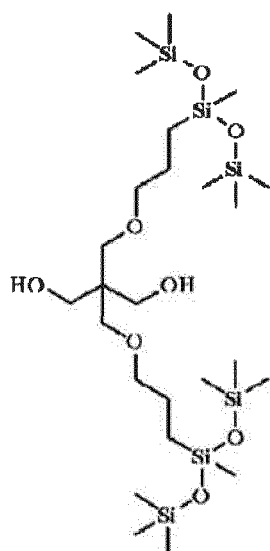
Silicon-containing compound-1
