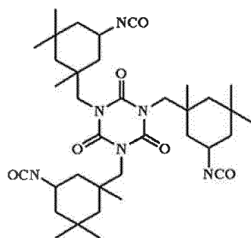
Isocyanate compound-4
