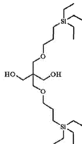
Silicon-containing compound-3
