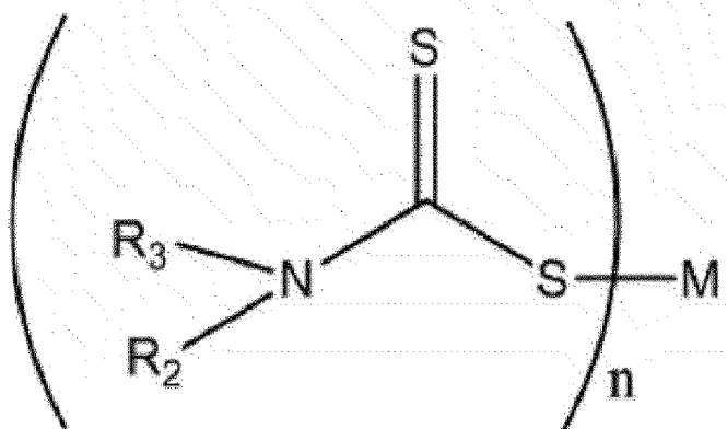
[Chemical Formula 3]
