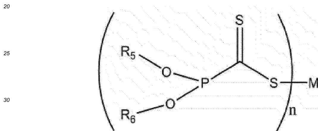
[Chemical Formula 4]
