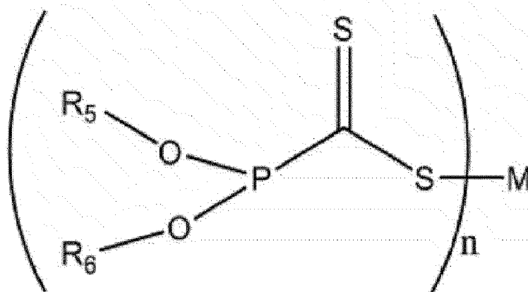
[Chemical Formula 4]
