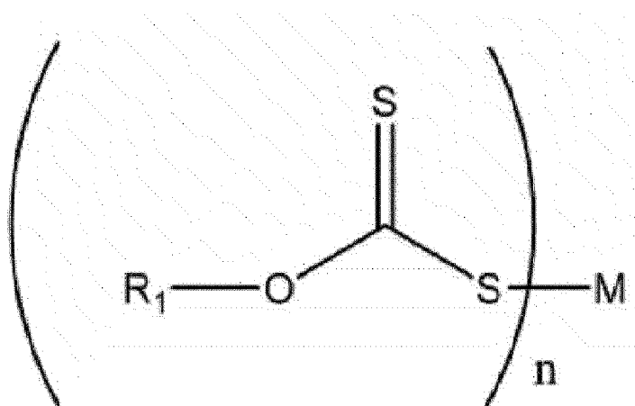
[Chemical Formula 2]
