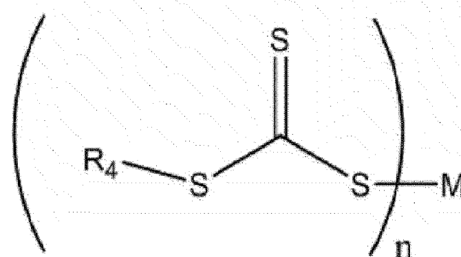
[Chemical Formula 4]
