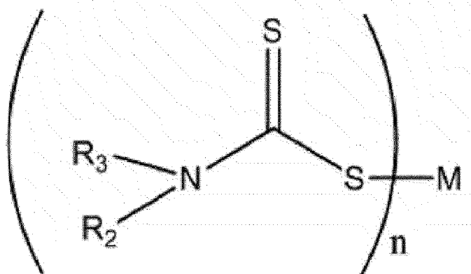
[Chemical Formula 2]
