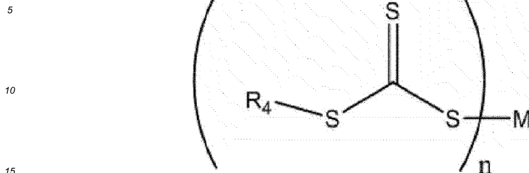
[Chemical Formula 4]
