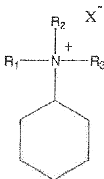
[Chem. 1]
