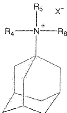
[Chem. 7]
