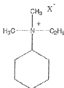
[Chem. 9]
