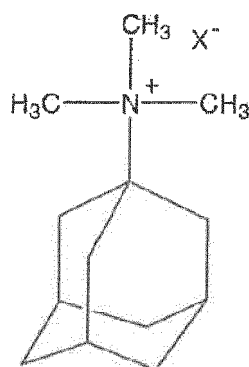
[Chem. 8]
