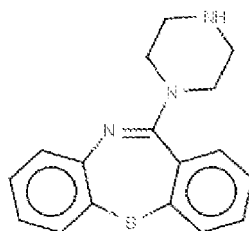
(norQTP)
