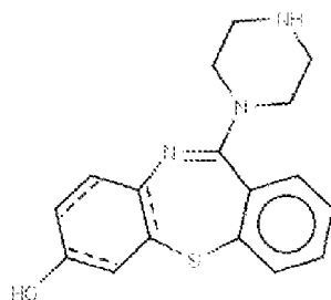
(7-OH-norQTP)
